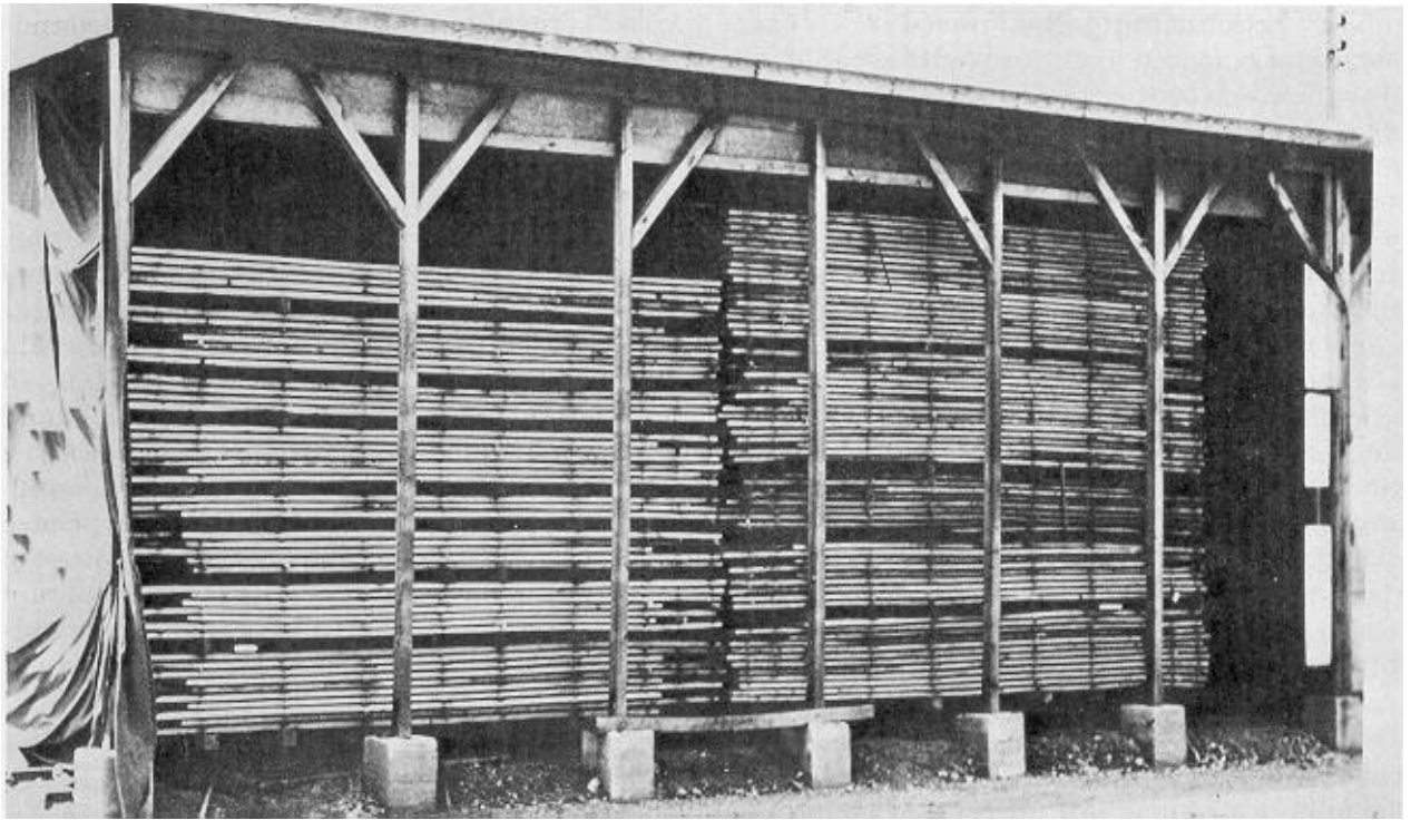
Figure 8.—Shed-fan track-type accelerated-air dryer.
