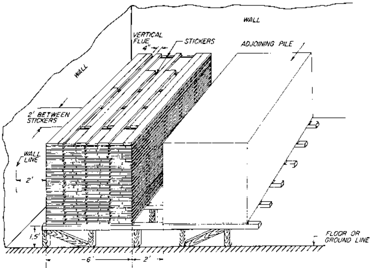
Figure 19.—Lumber piled for drying in a heated room.
