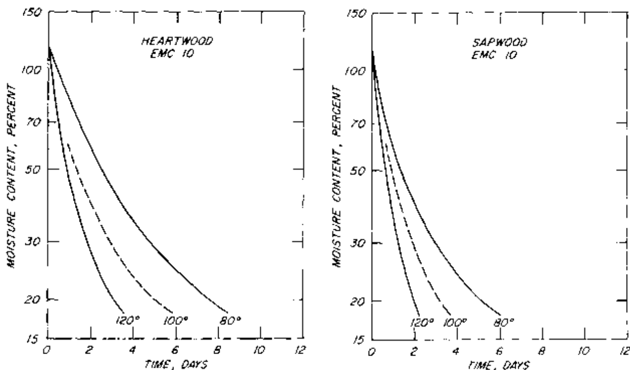
Figure 7.—Effect of temperature on drying of 1-inch yellow-poplar lumber in a low-temperature forced-air dryer under 10 percent EMC conditions (after Vick 1965b). M 144694
