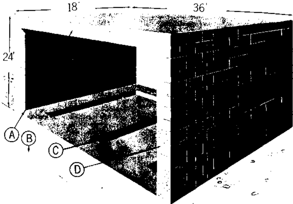
Figure 16.—Steaming chamber constructed of concrete block and poured, reinforced concrete: A, Roof is poured concrete or prestressed concrete sections; B, apron or loading ramp; C, trough for perforated or imperforated steam pipes in water; and D, walls of concrete blocks or poured concrete.
