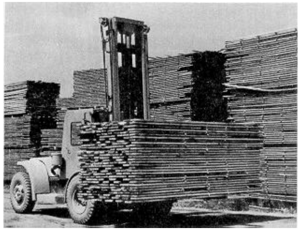
Figure 3.—Stacking stickered package of lumber.
