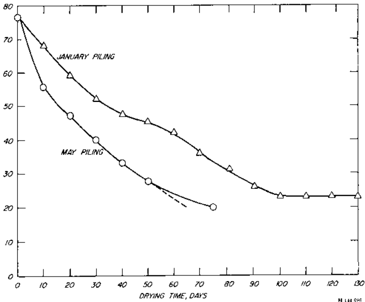
Figure 6.—Air drying curves for 4/4 northern red oak piled at different times of year in southern Wisconsin.
