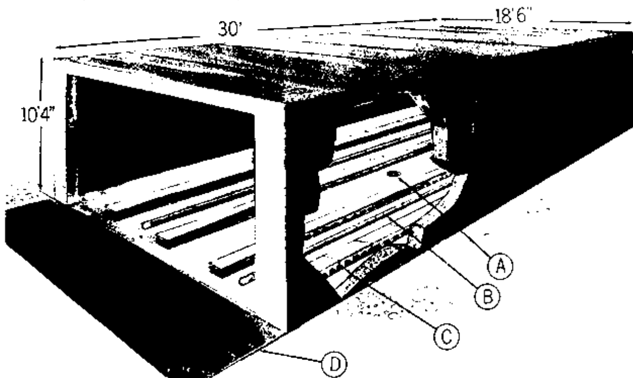
Figure 17.—Steaming vat of wood and sheet aluminum construction (Details courtesy of Hartzell Industries, Inc., Piqua, Ohio): A, Sheet aluminum lining, with joints sealed with asphaltic materials; B, roof sections of creosoted frame and planks, lined with sheet aluminum; sections are placed by forklift truck as vat is filled; C, trough for perforated steam pipes in water; D, slanted jamb causes door sections to fit securely by weight alone; E, creosoted posts set in ground; and F, creosoted 2- by 8-inch plank wall.
