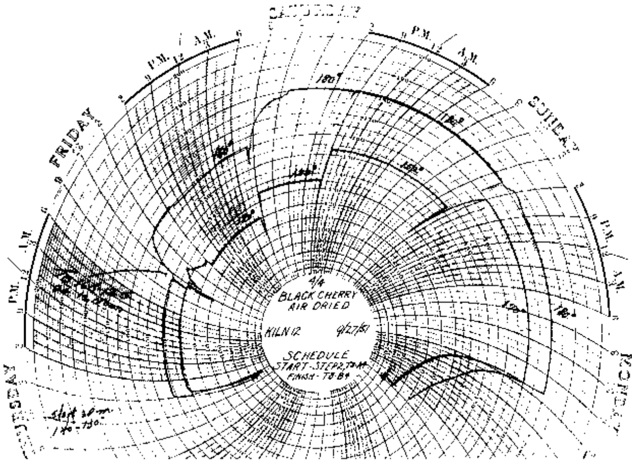
Figure 12.—Instrument chart of conditions used in kiln drying a small load of air-dried black cherry. (Assumed to have undergone surface moisture regain.)
