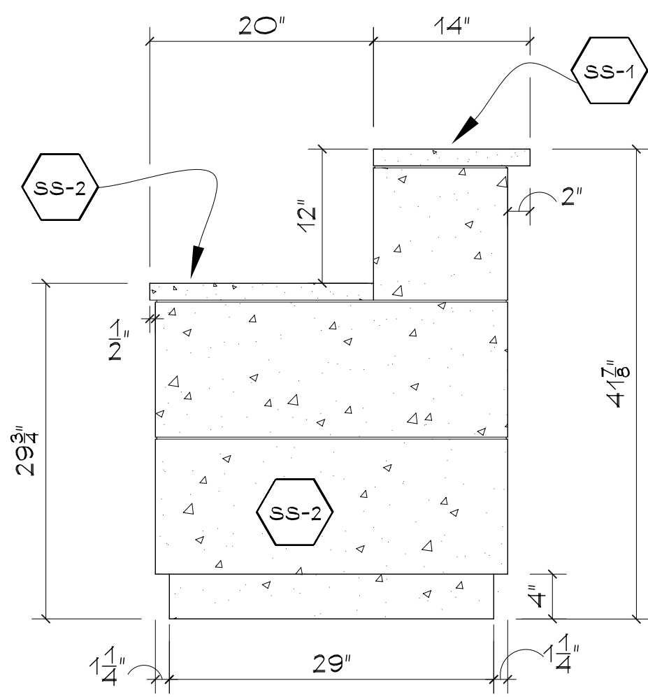
1 ELEVATION SC. 1/4"=1'-0"
