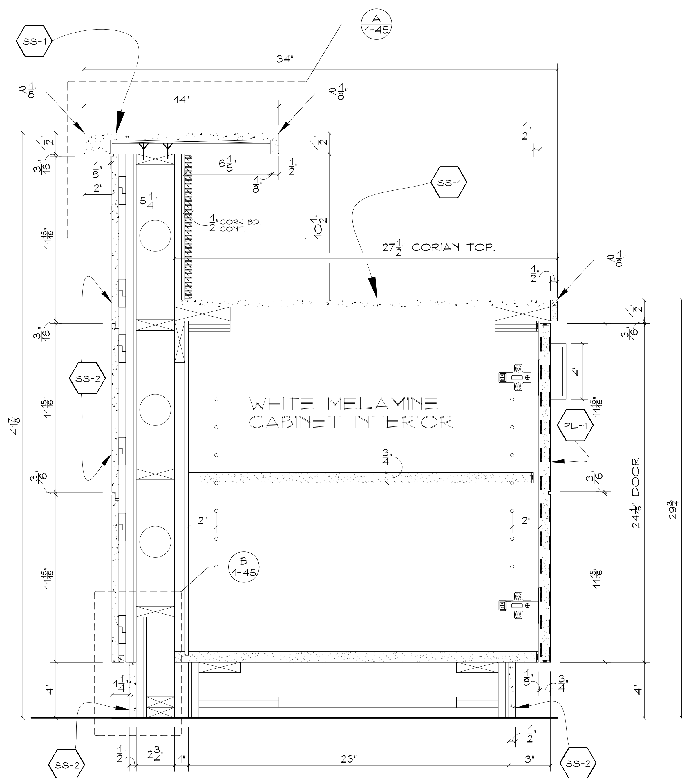
2 SECTION SC. 3/4"=1'-0"
