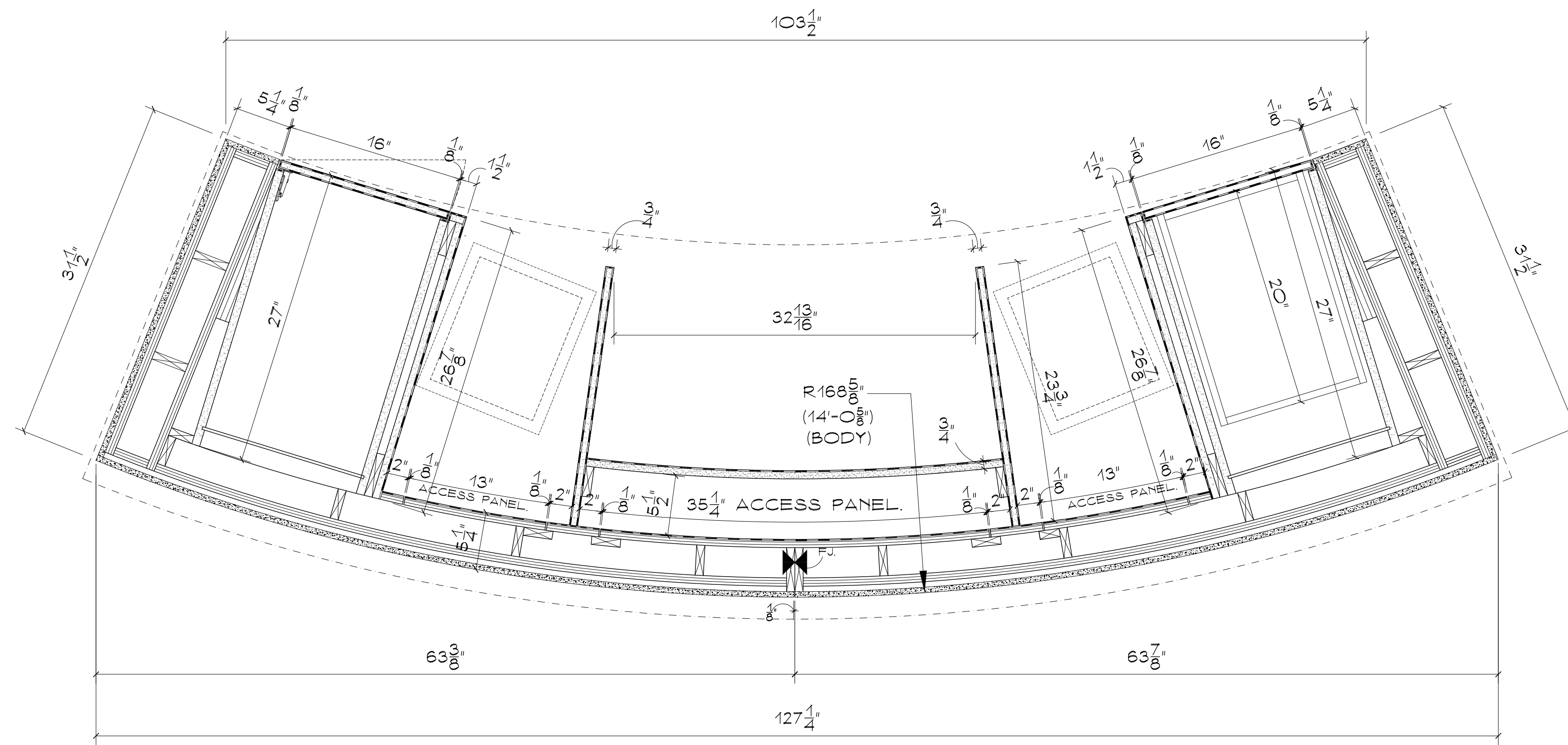
1 PLAN SECTION SC. 1 1/2"=1'-0"
