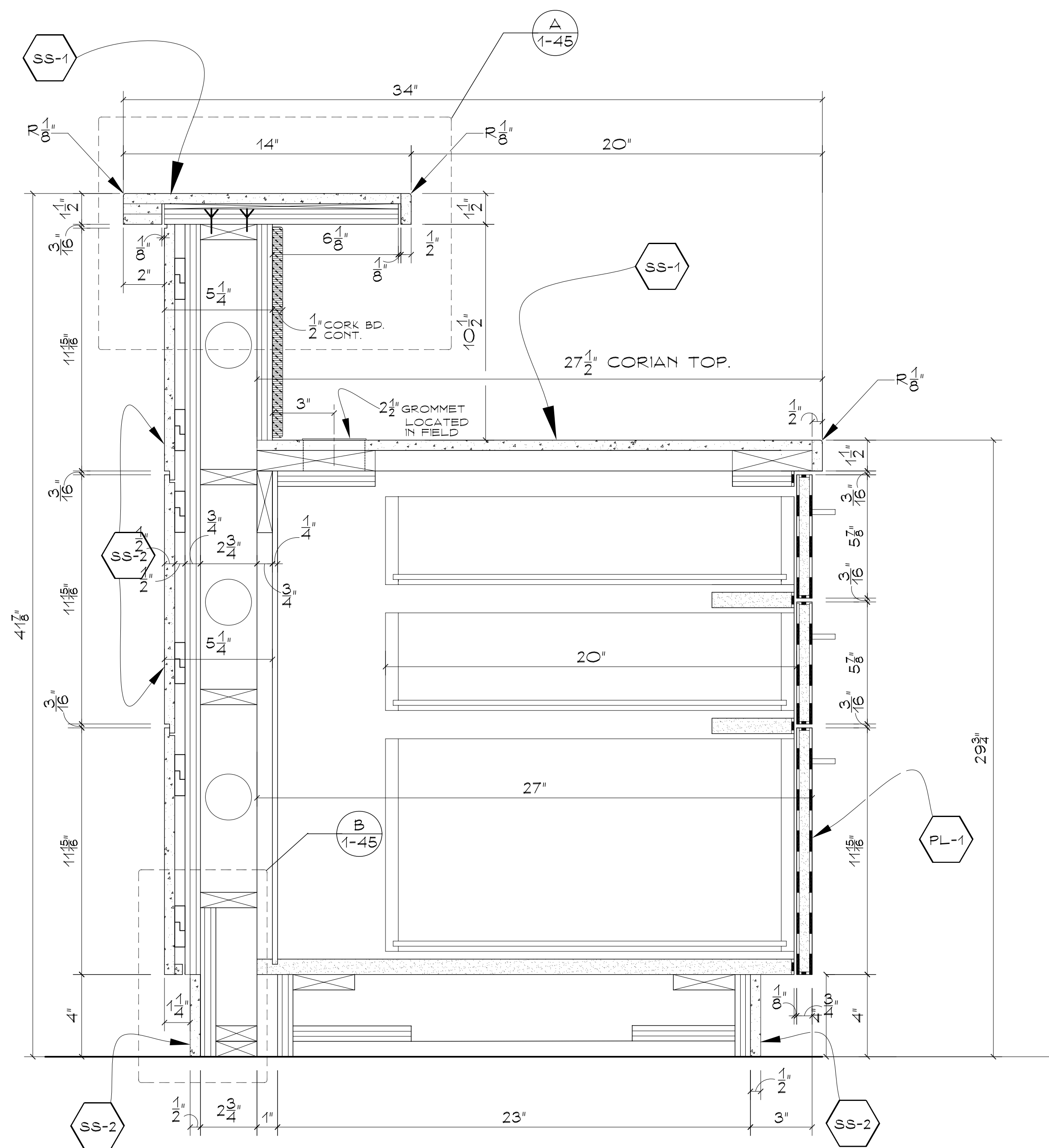
1 SECTION SC. 3/4"=1'-0"
