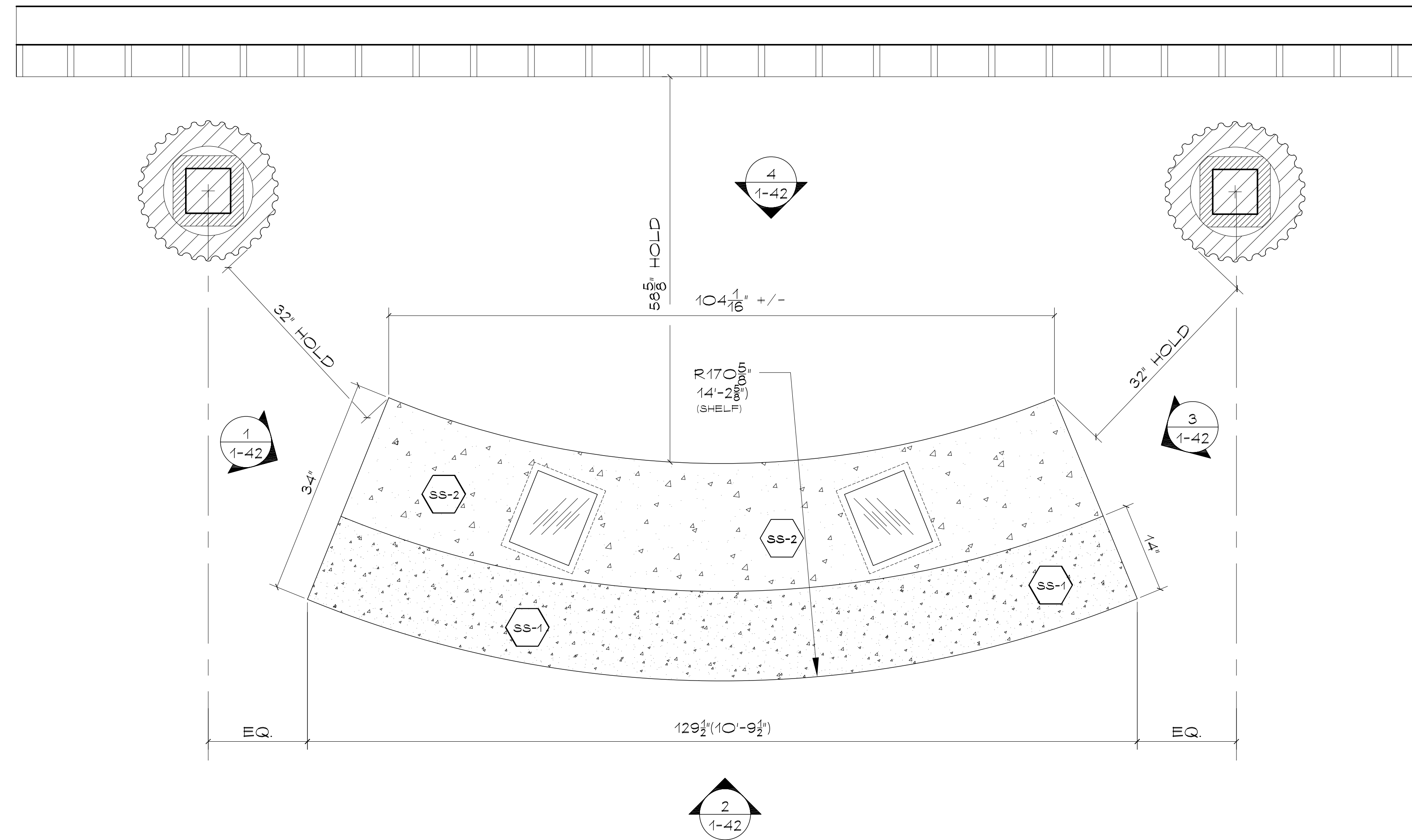
1 PLAN SC. 1/4"=1'-0"
