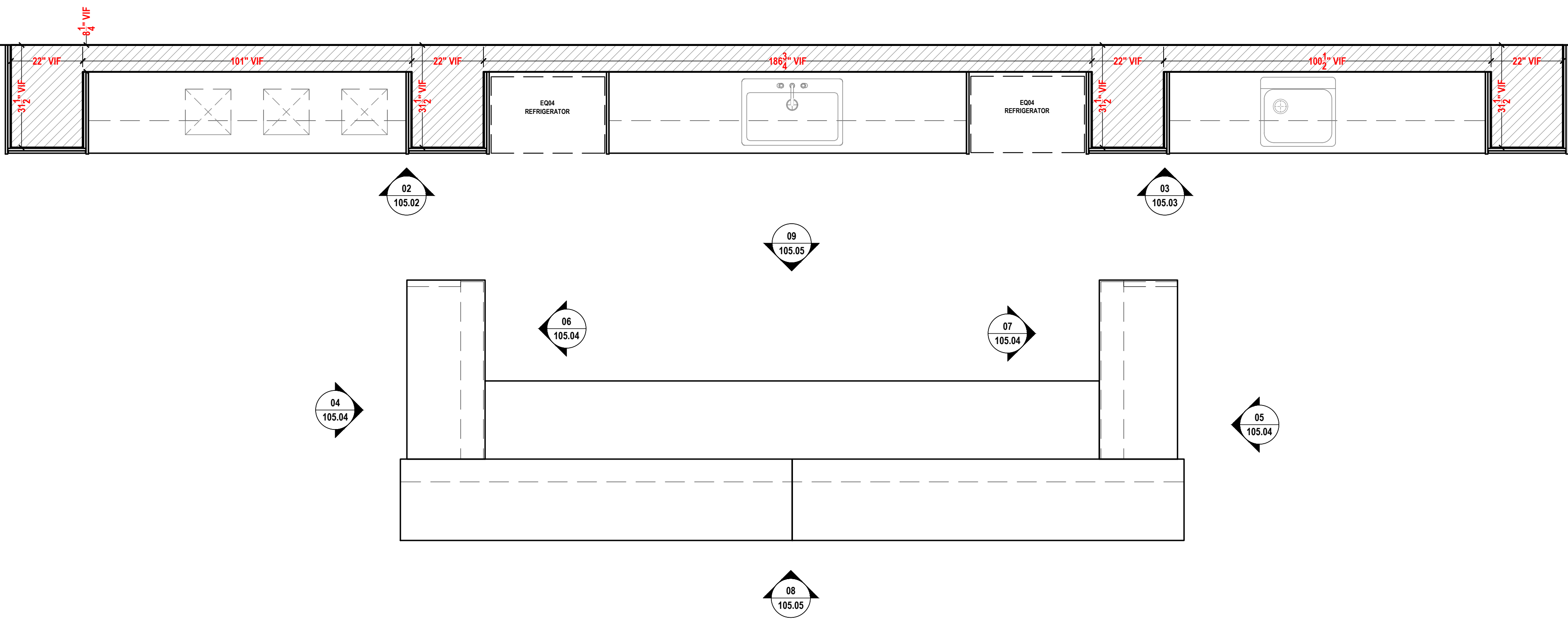
01 BREAK ROOM A204 PLAN VIEW SCALE: 1/2"=1'-0" ARCH REF.: A1/A608
