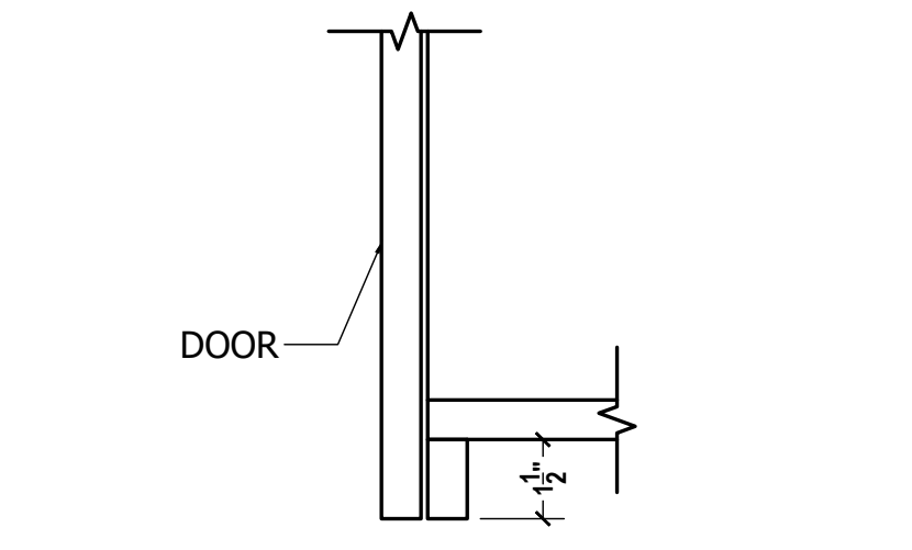
N FILLER AT WALL DETAIL SCALE: 3"=1'-0" ARCH REF.:
