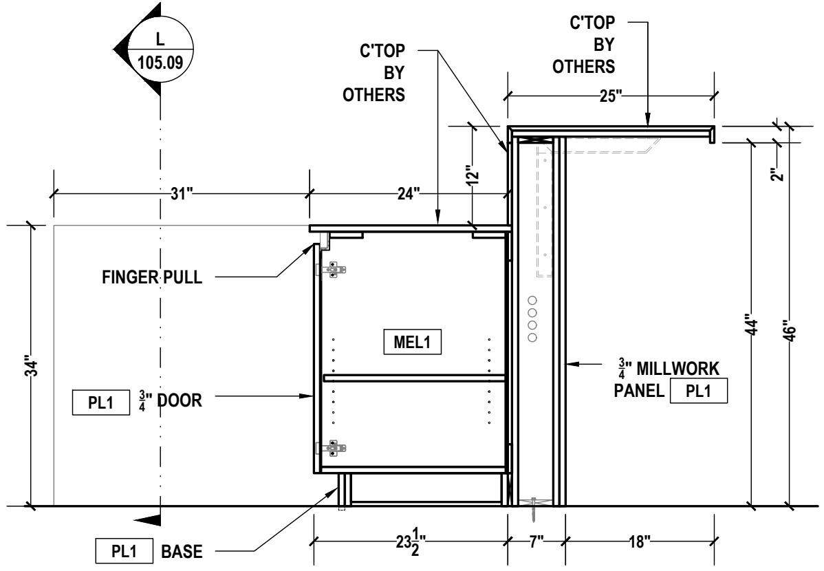
07 BREAK ROOM A204 ELEVATION SCALE: 3/4"=1'-0" ARCH REF.: A7/A608
