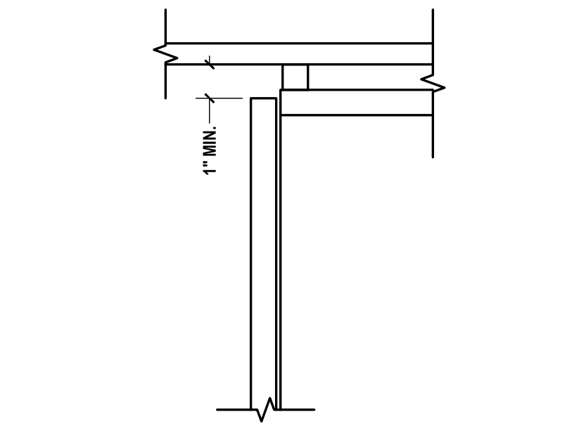
E CEILING FILLER DETAIL SCALE: 3"=1'-0" ARCH REF.:
