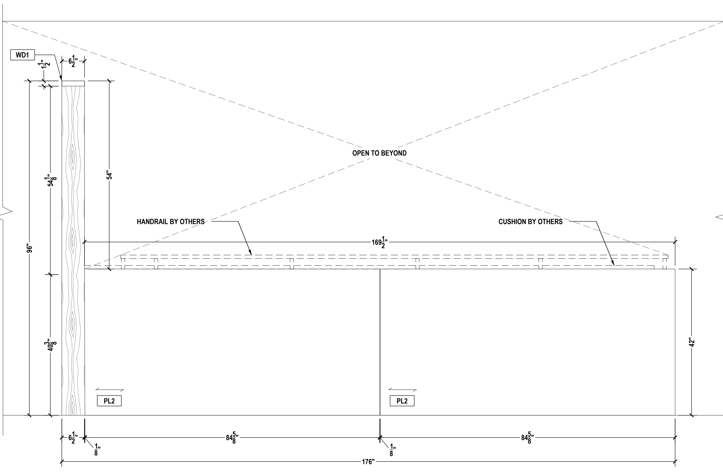
03 LOUNGE A103 - BANQUETTE ELEVATION SCALE: 3/4"=1'-0" ARCH REF.: A3/A603
