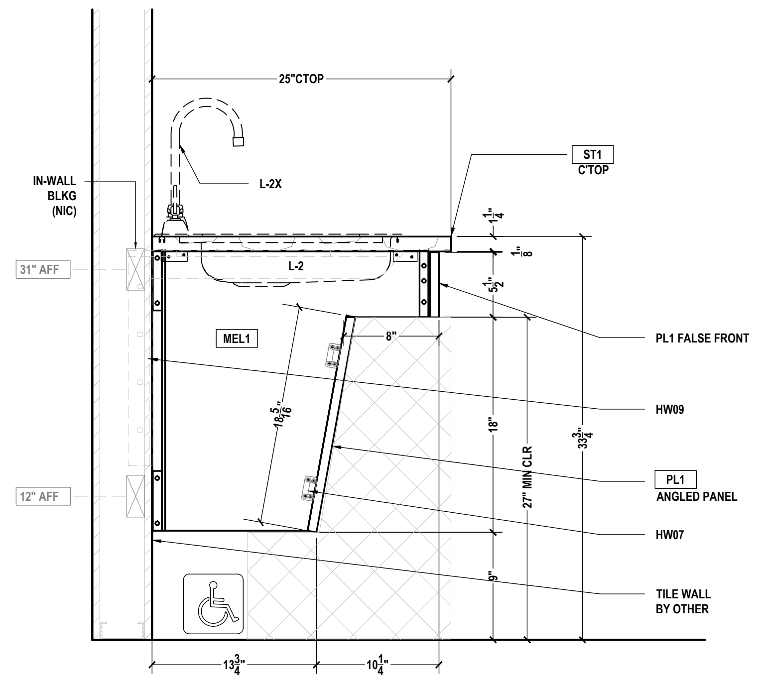
B RESTROOMS A402 SECTION SCALE: 1-1/2"=1'-0" ARCH REF.: 19/A604B
