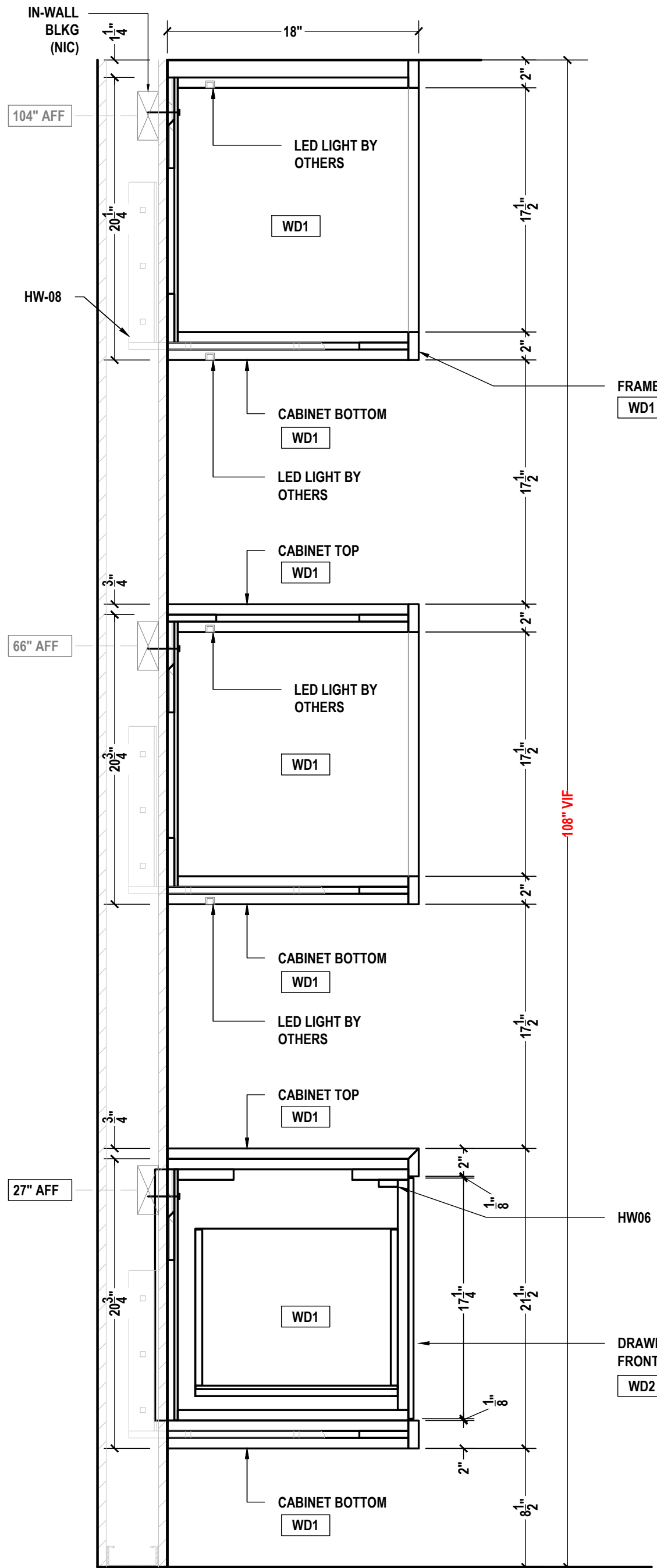
A LOBBY A105 SECTION SCALE: 1-1/2"=1'-0" ARCH REF.: 15/A604B
