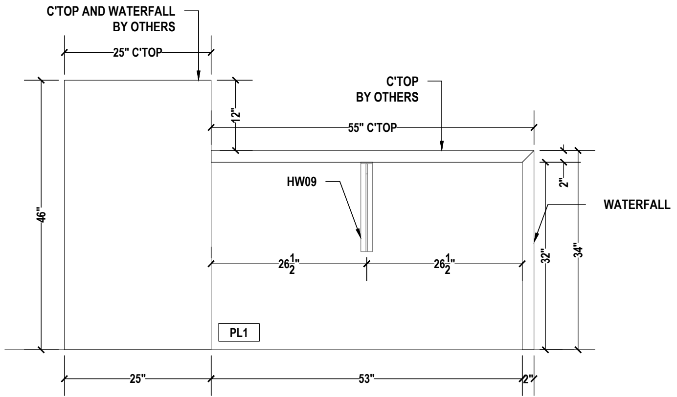
05 BREAK ROOM A204 ELEVATION SCALE: 3/4"=1'-0" ARCH REF.: A4/A608
