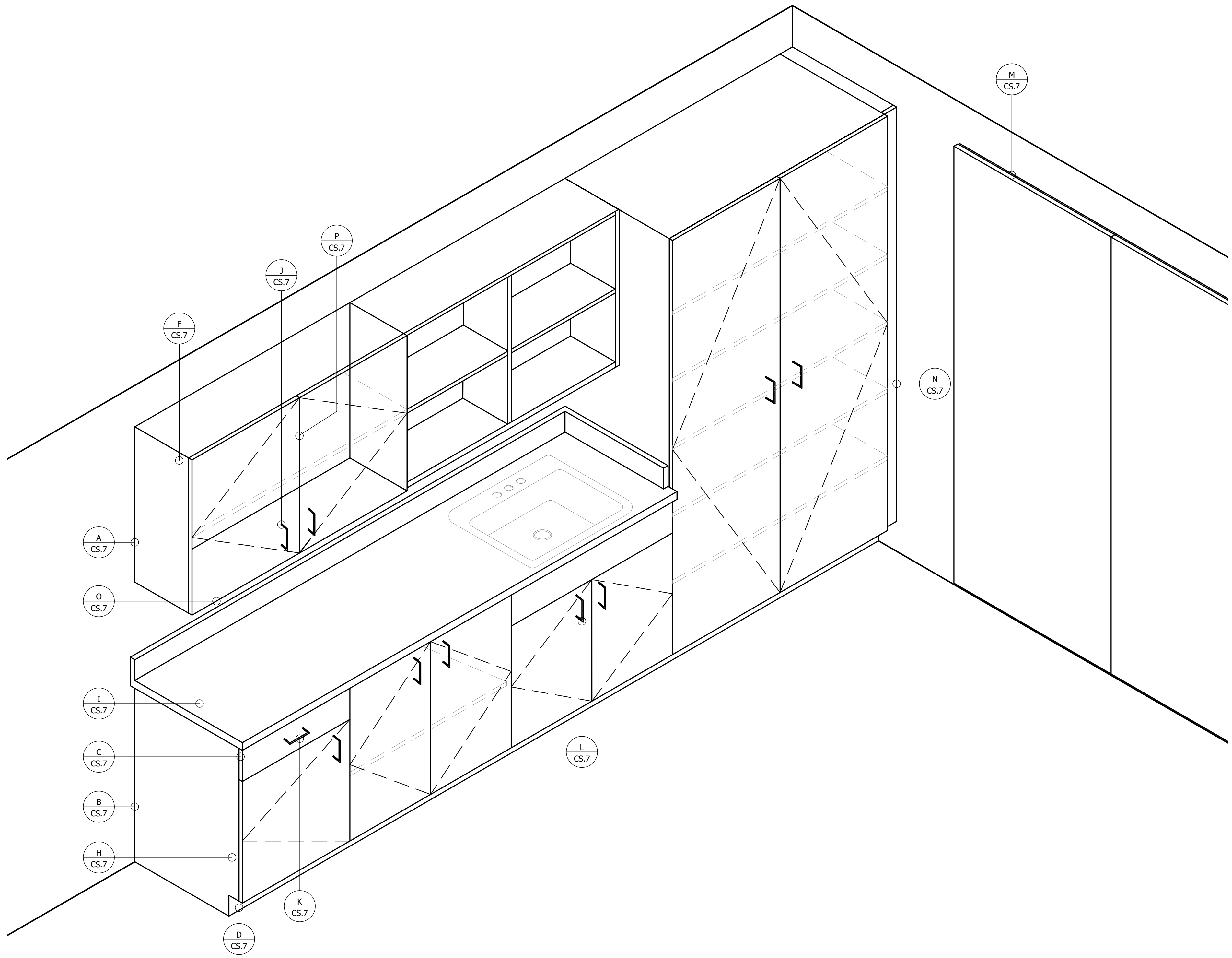
01 TYPICAL CONSTRUCTION AXONOMETRIC AXONOMETRIC SCALE: ARCH REF.:
