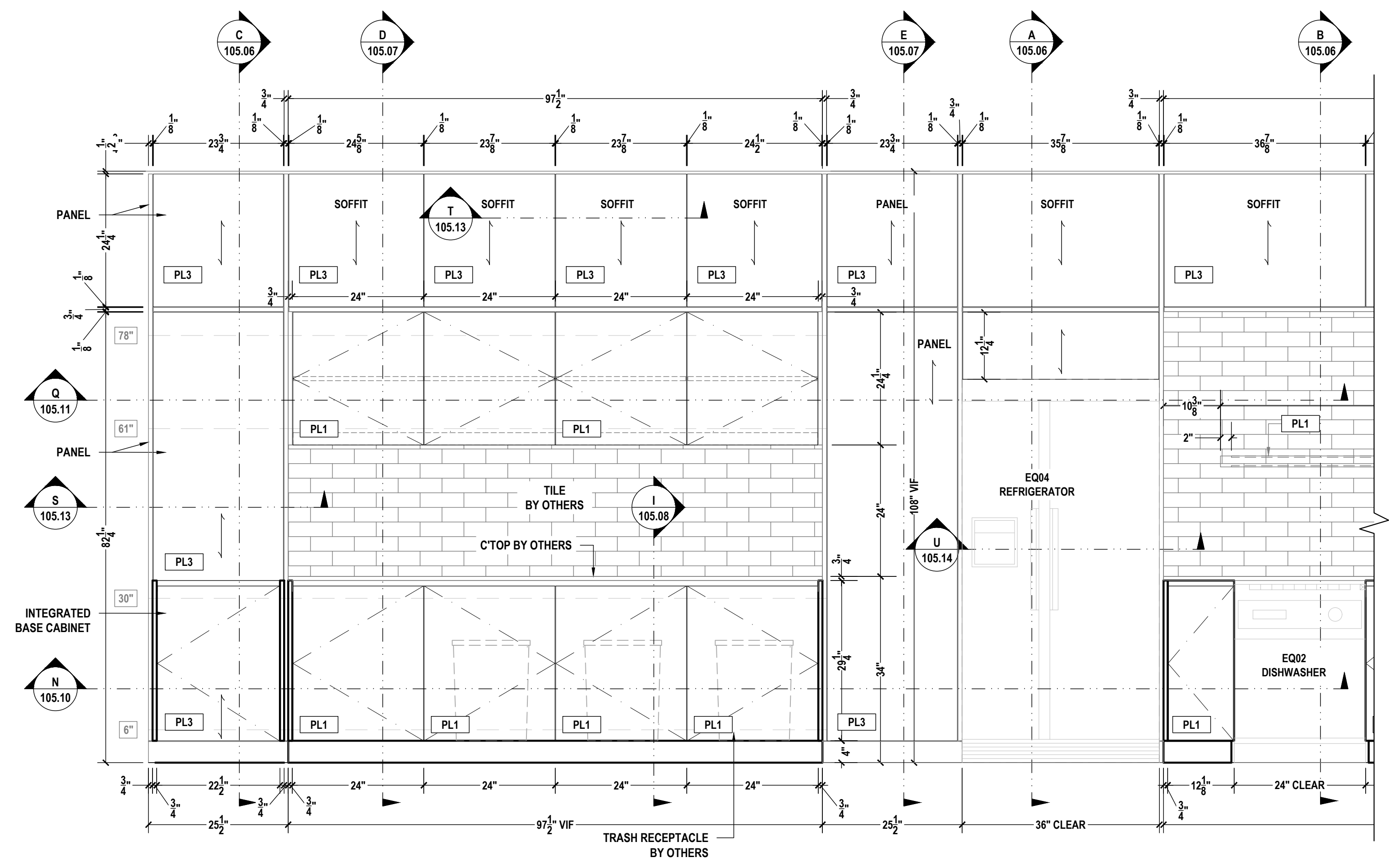
02 BREAK ROOM A204 ELEVATION SCALE: 3/4"=1'-0" ARCH REF.: A2/A608
