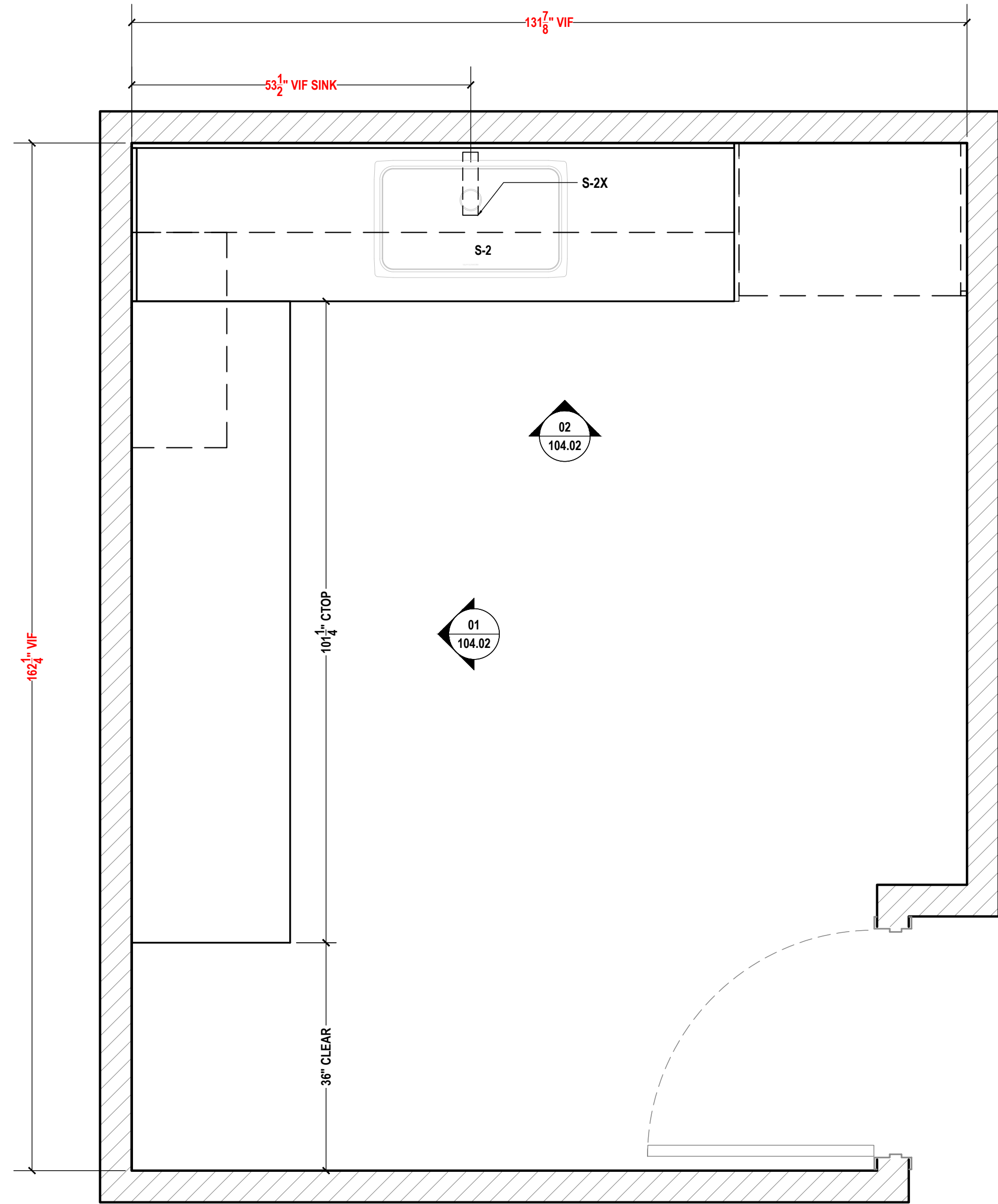
01 WORKING ROOM A108 PLAN VIEW SCALE: 3/4"=1'-0" ARCH REF.: A1/A607
