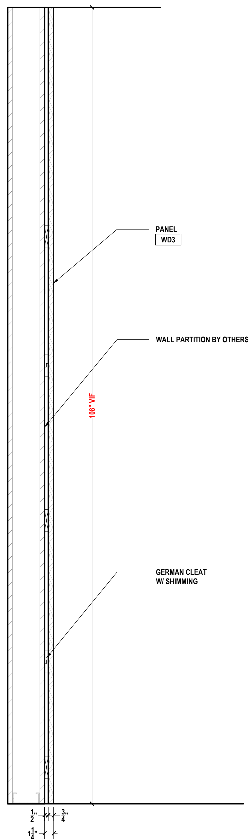
A RESTROOMS A402 SECTION SCALE: 1-1/2"=1'-0" ARCH REF.: 18/A604B
