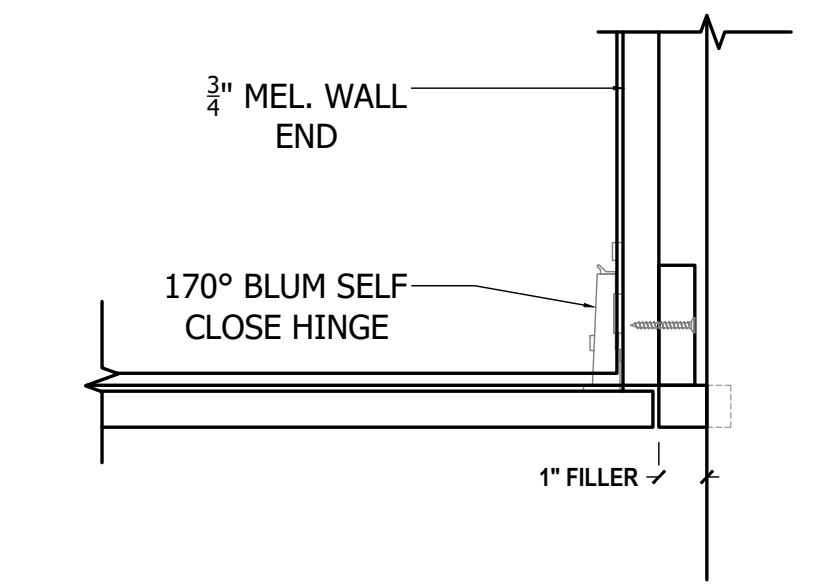
N FILLER AT WALL DETAIL SCALE: 3"=1'-0" ARCH REF.:
