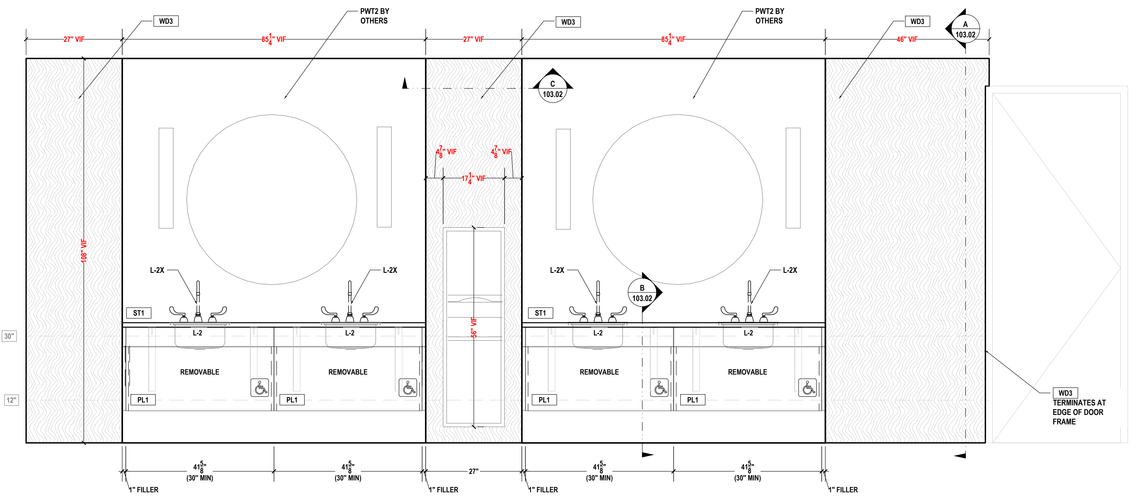
02 RESTROOMS A402 ELEVATION SCALE: 3/4"=1'-0" ARCH REF.: A14/A606
