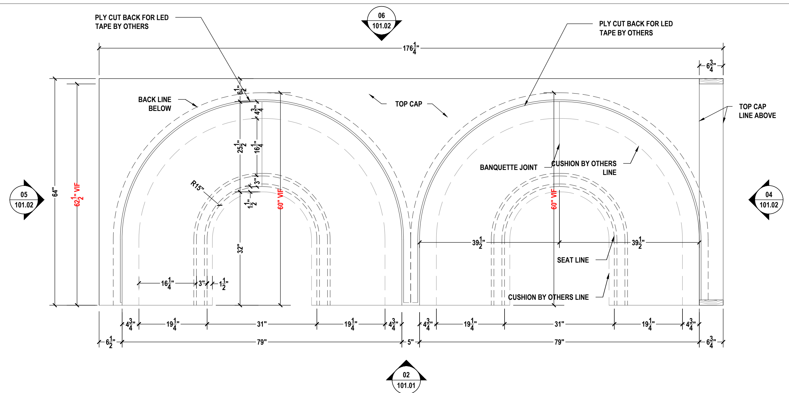
01 LOUNGE A103 - BANQUETTE PLAN VIEW SCALE: 3/4"=1'-0" ARCH REF.: A1/A603
