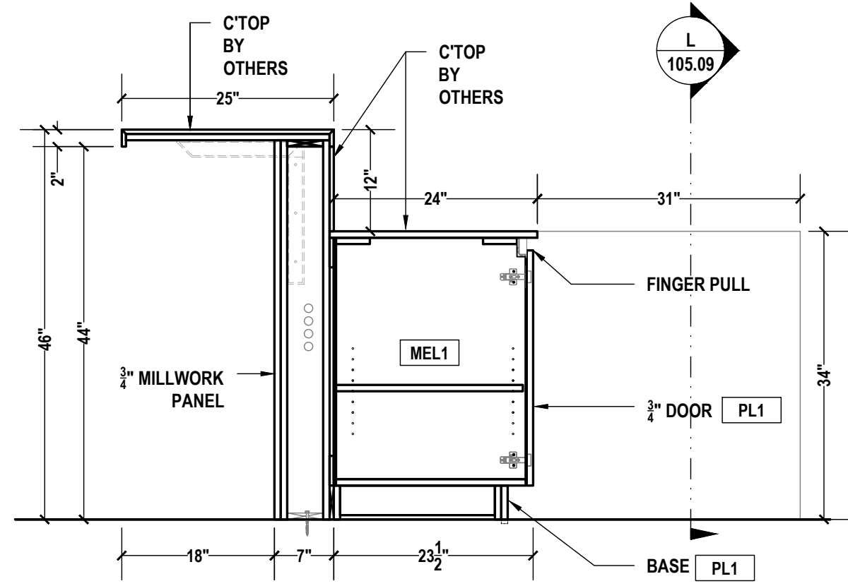
06 BREAK ROOM A204 ELEVATION SCALE: 3/4"=1'-0" ARCH REF.: A6/A608
