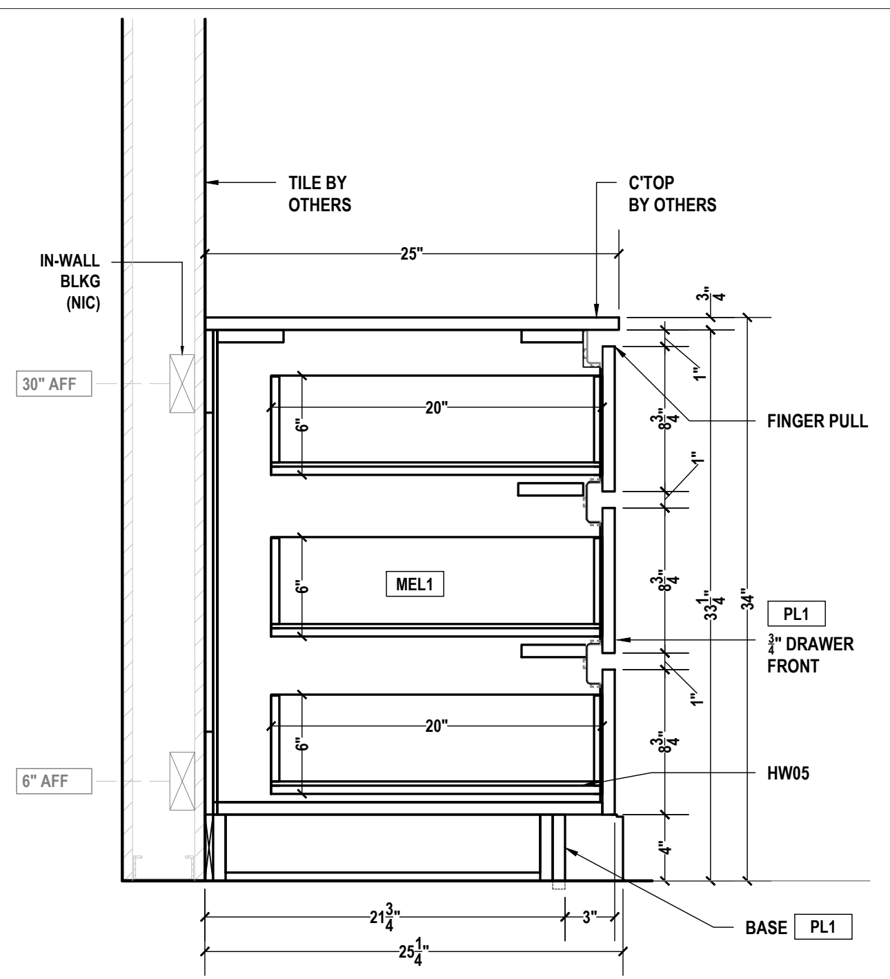
G BREAK ROOM SECTION SCALE: 1-1/2"=1'-0" ARCH REF.: 16/A605B
