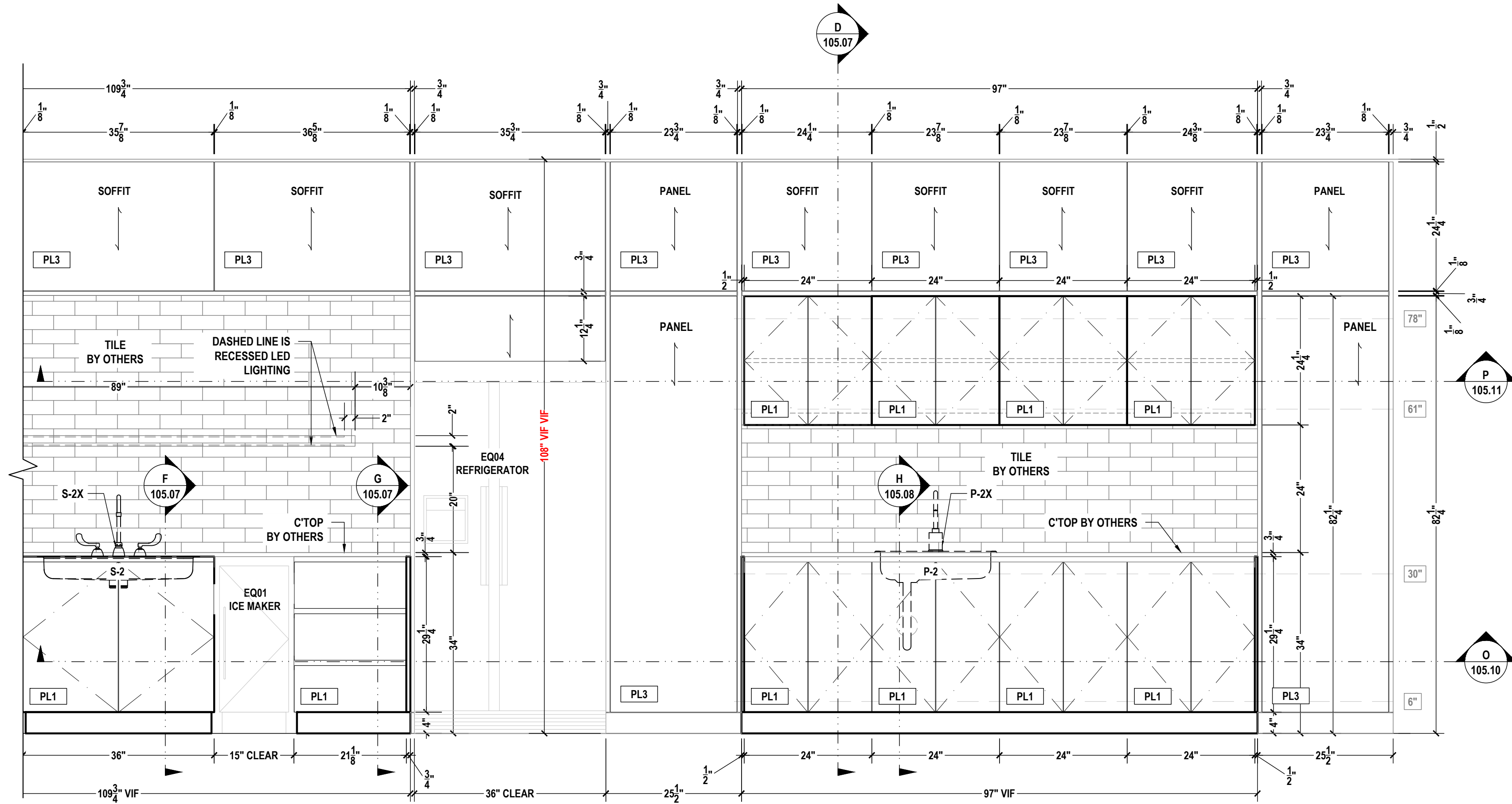
03 BREAK ROOM A204 ELEVATION SCALE: 3/4"=1'-0" ARCH REF.: A2/A608
