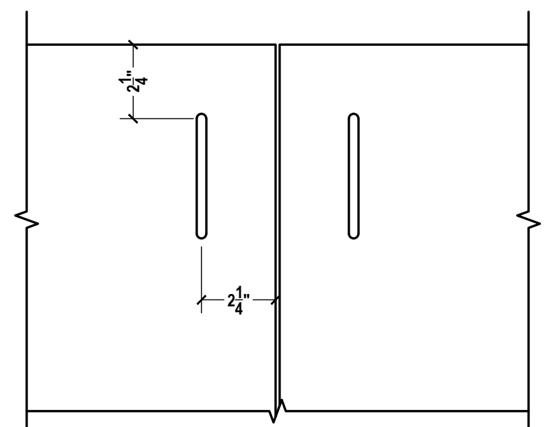
L BASE DOOR PULL LOCATION DETAIL SCALE: 3"=1'-0" ARCH REF.:
