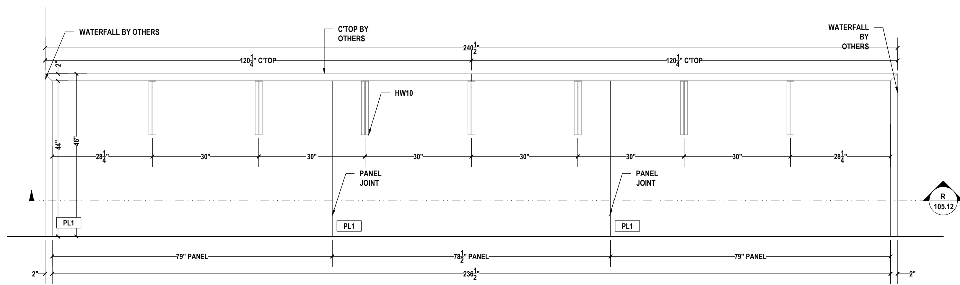
08 BREAK ROOM A204 ELEVATION SCALE: 3/4"=1'-0" ARCH REF.: A5/A608
