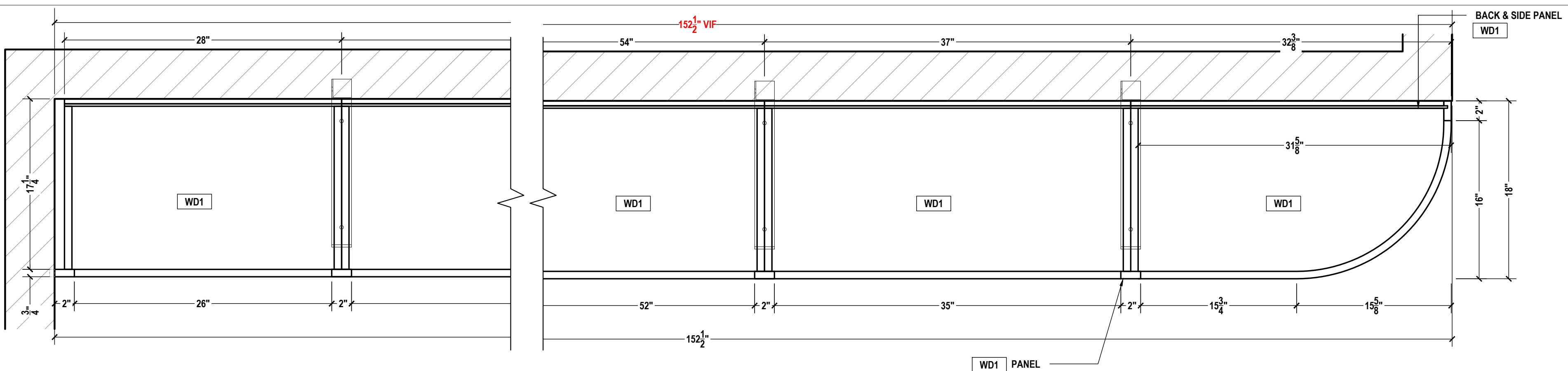
D LOBBY A105 HORIZONTAL SECTION SCALE: 1-1/2"=1'-0" ARCH REF.: N/A
