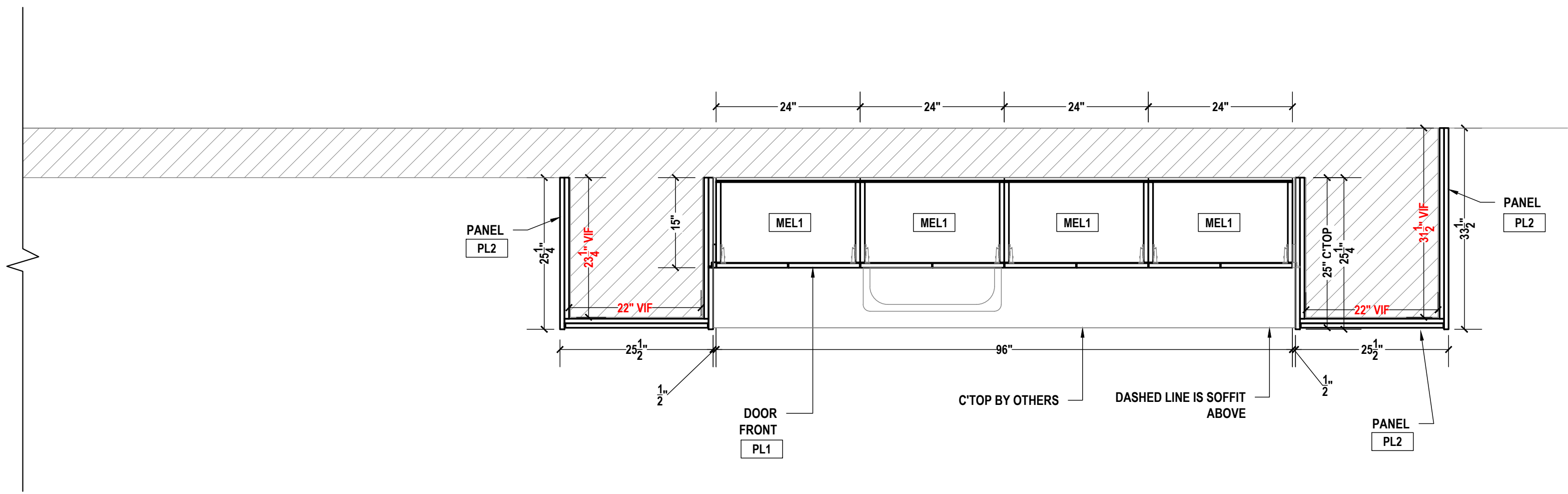
P BREAK ROOM A204 HORIZONTAL SECTION SCALE: 3/4"=1'-0" ARCH REF.: N/A
