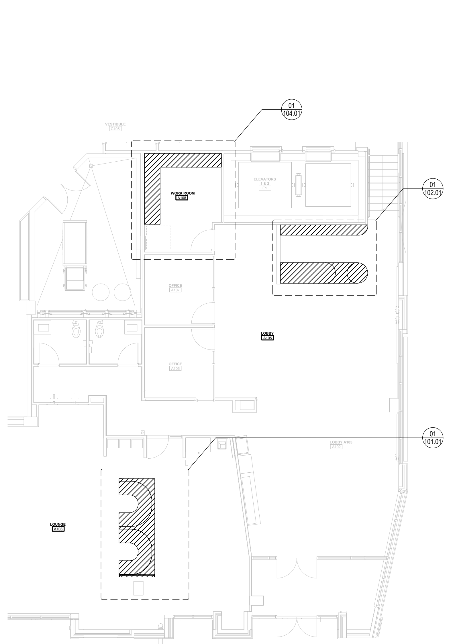
03 LEVEL 1 ENLARGED PLAN - LOBBY A105 REFERENCE PLAN SCALE: 1/8"=1'-0" ARCH REF.: A1/A601A
