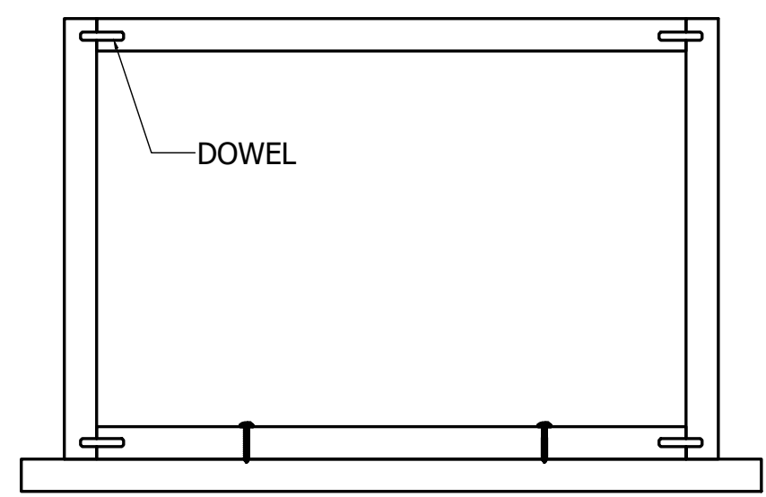
C DRAWER CONSTRUCTION DETAIL SCALE: 3"=1'-0" ARCH REF.:
