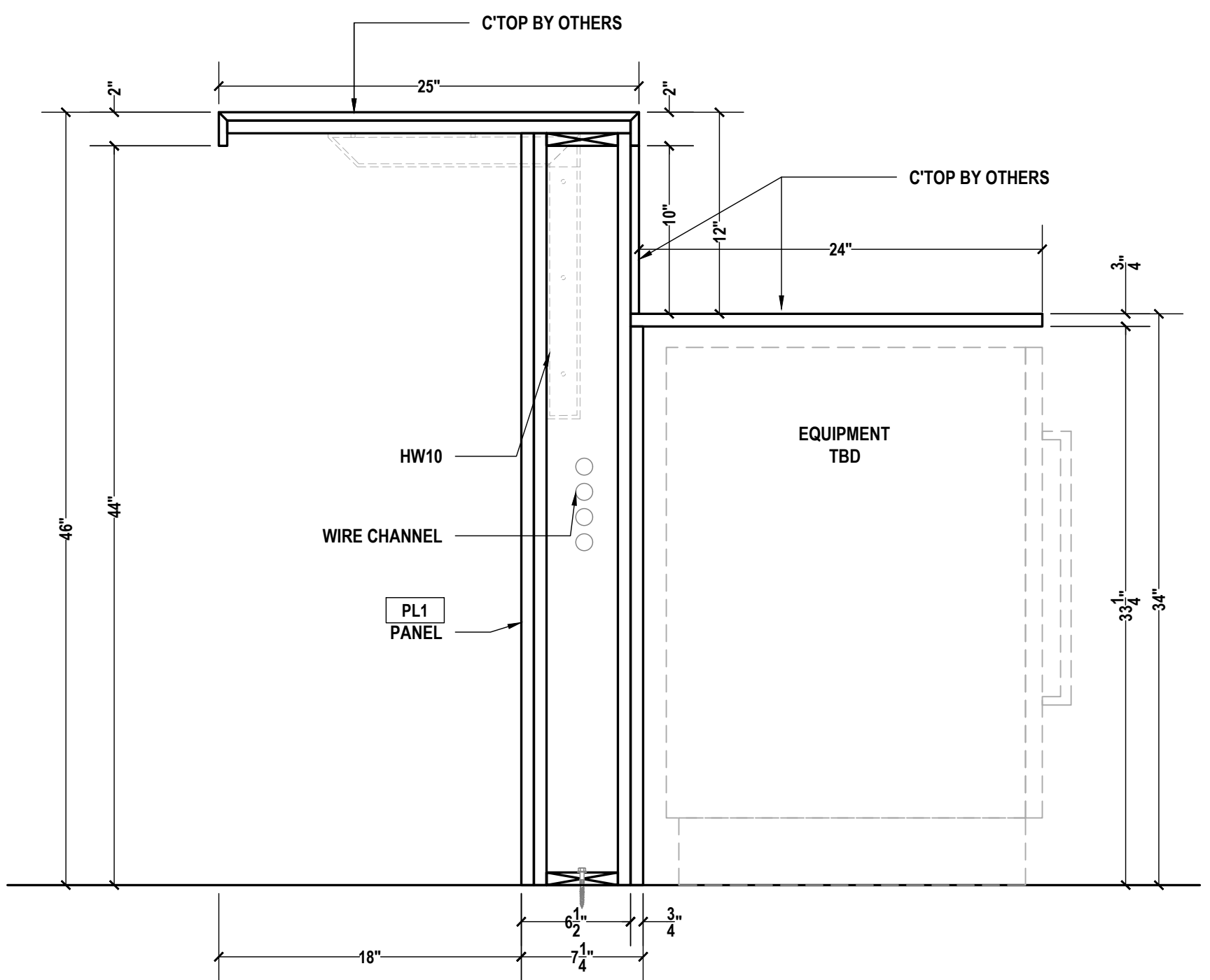
J BREAK ROOM SECTION SCALE: 1-1/2"=1'-0" ARCH REF.: 19/A605B
