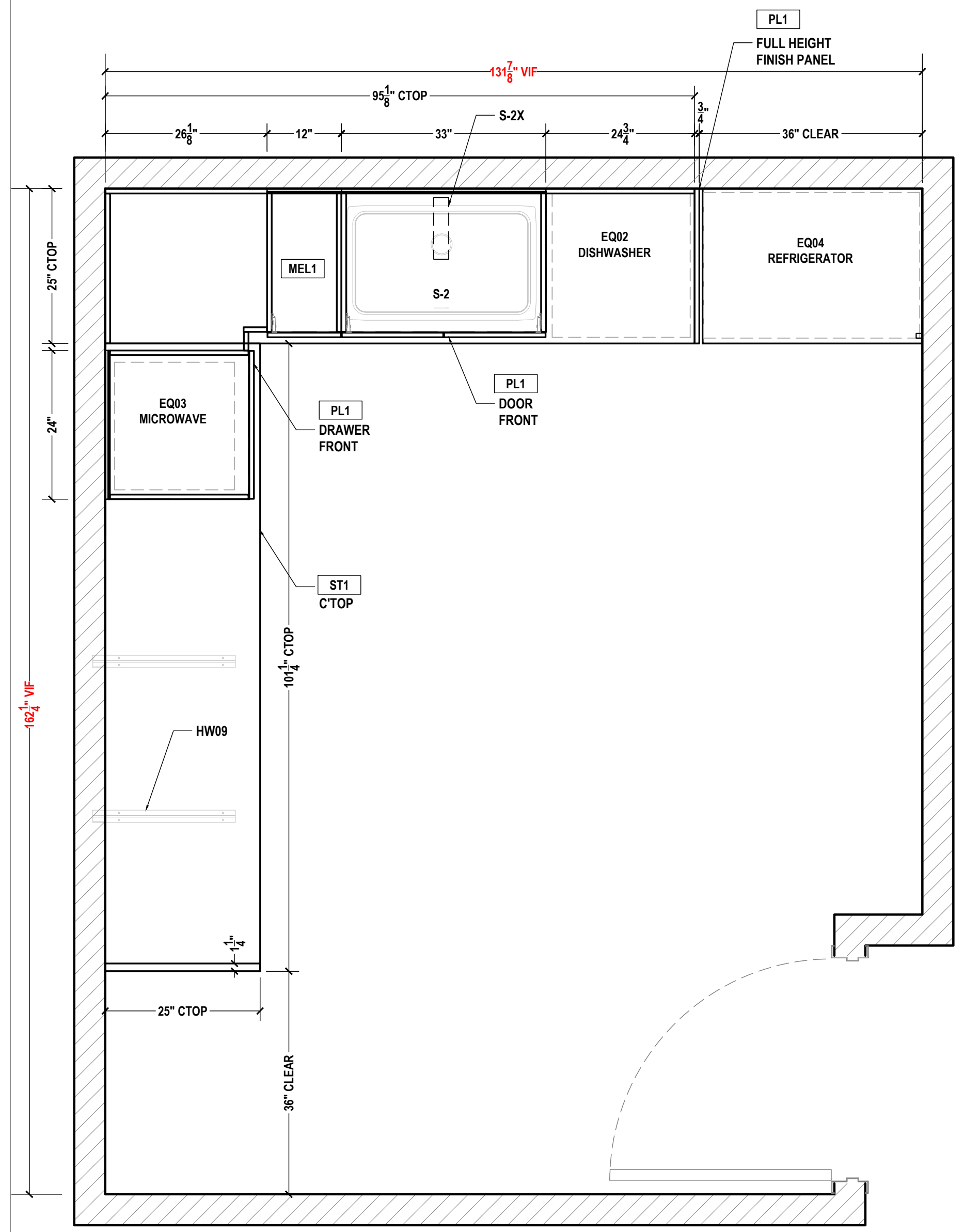
G WORKING ROOM A108 HORIZONTAL SECTION SCALE: 3/4"=1'-0" ARCH REF.: N/A
