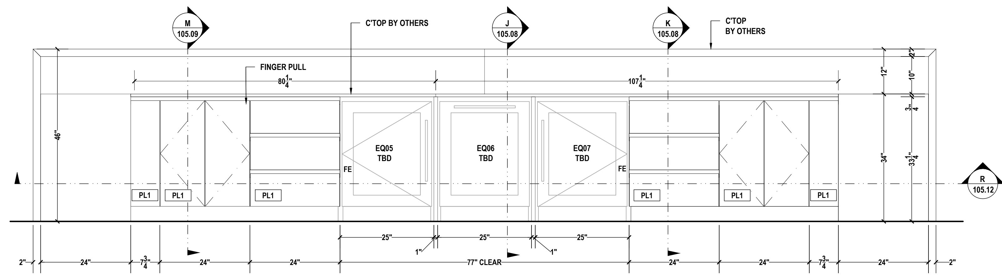
09 BREAK ROOM A204 ELEVATION SCALE: 3/4"=1'-0" ARCH REF.: A8/A608
