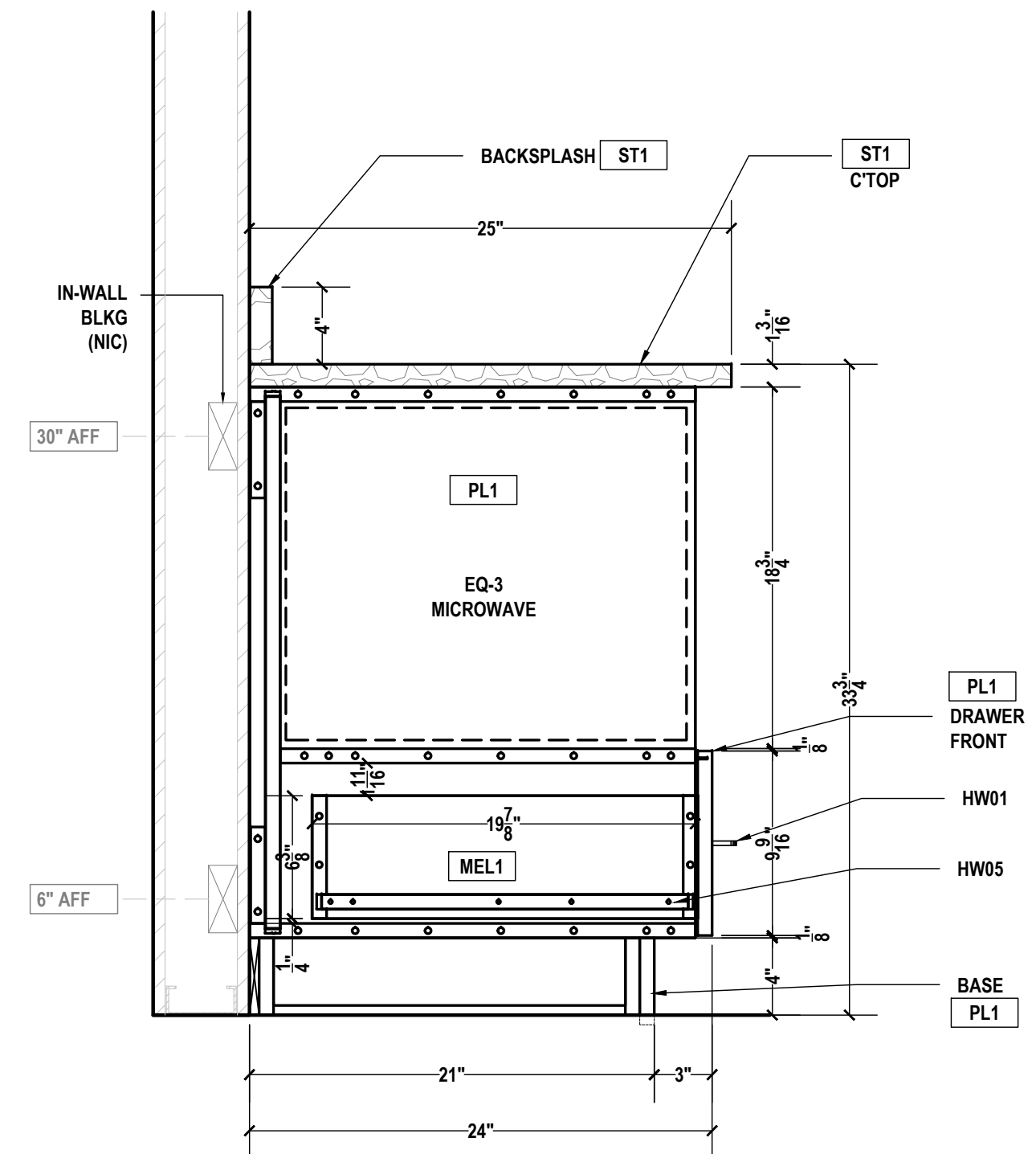
F WORKING ROOM A108 SECTION SCALE: 1-1/2"=1'-0" ARCH REF.: 26/A604B
