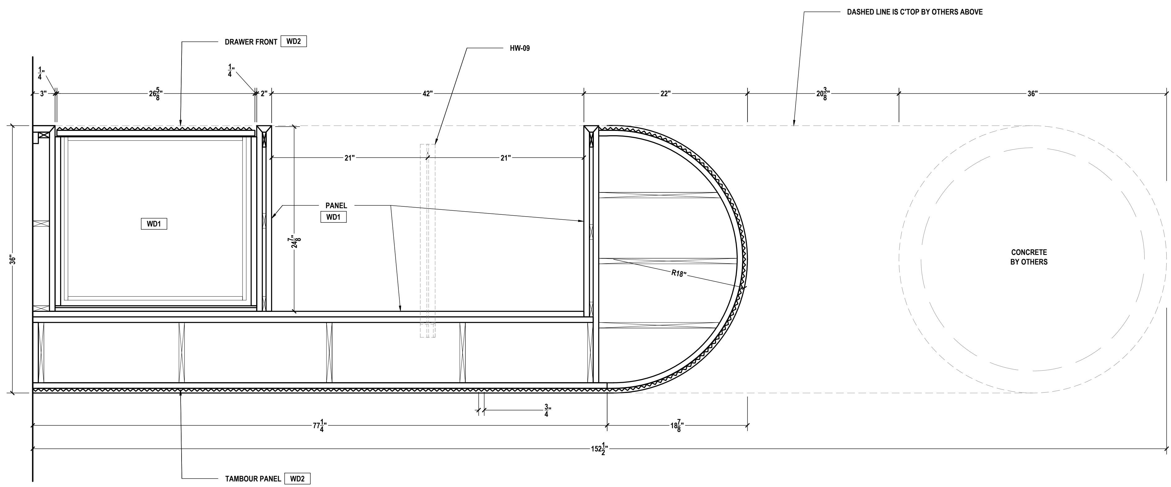
G LOBBY A105 HORIZONTAL SECTION SCALE: 1-1/2"=1'-0" ARCH REF.: N/A
