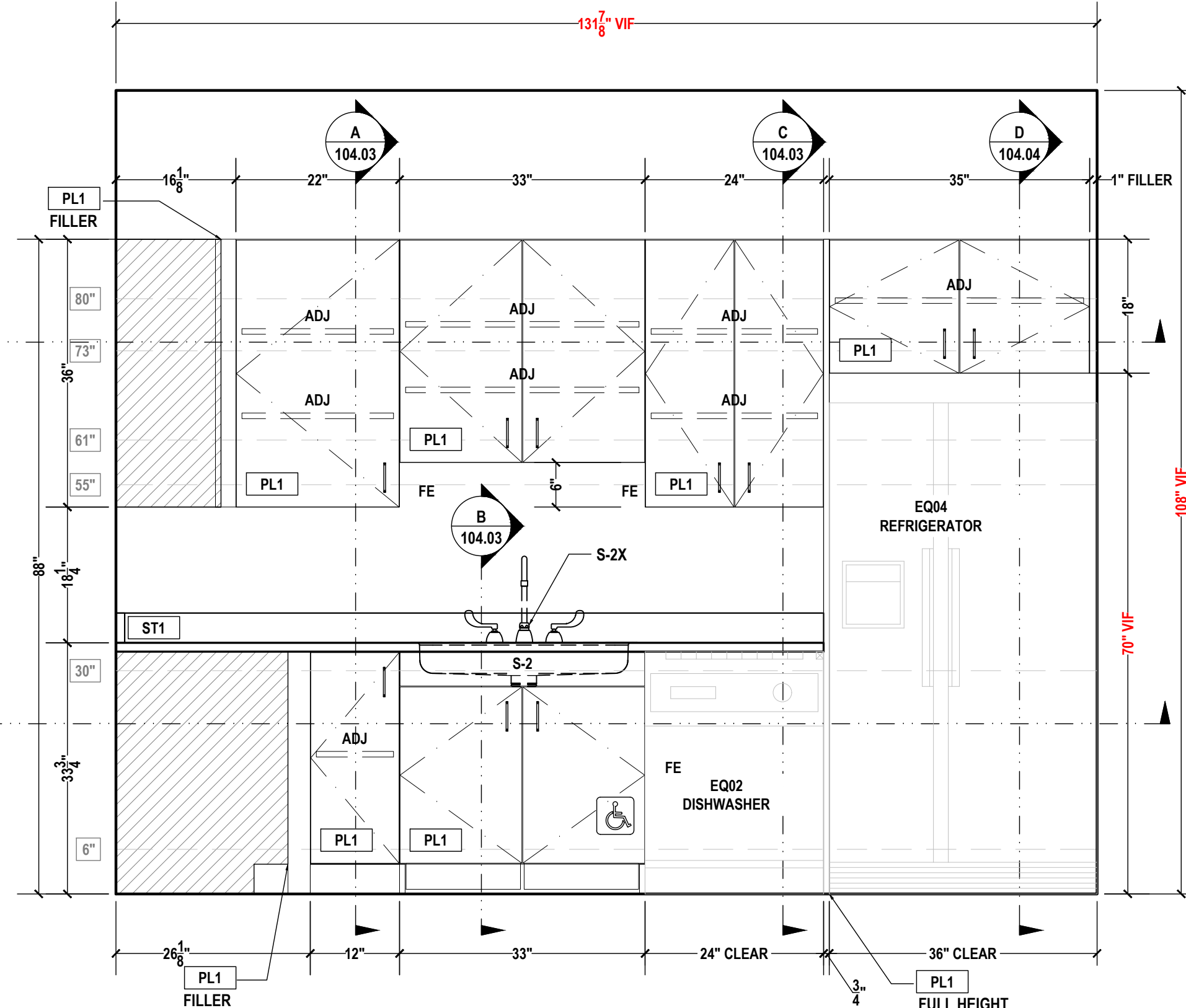
02 WORKING ROOM A108 ELEVATION SCALE: 3/4"=1'-0" ARCH REF.: A2/A607
