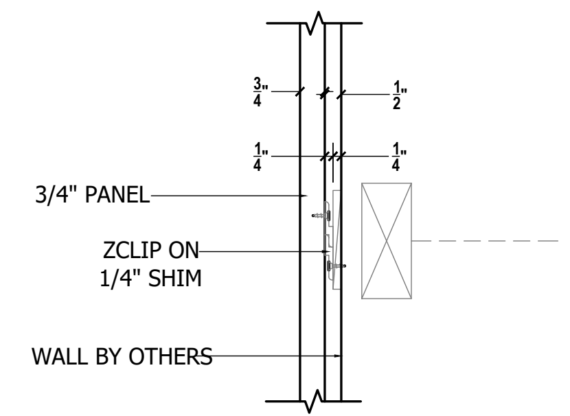
M WALL PANELING ANCHORAGE DETAIL SCALE: 3"=1'-0" ARCH REF.:
