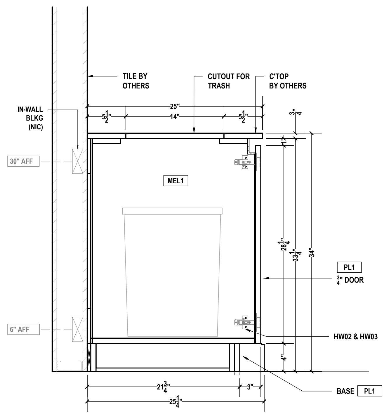
I BREAK ROOM SECTION SCALE: 1-1/2"=1'-0" ARCH REF.: 18/A605B
