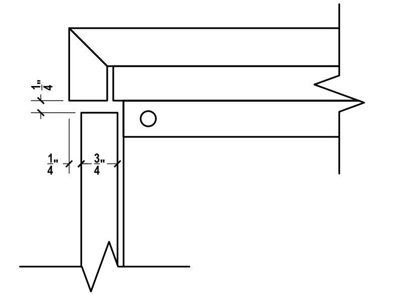
I C TOP DETAIL SCALE: 6"=1'-0" ARCH REF.:
