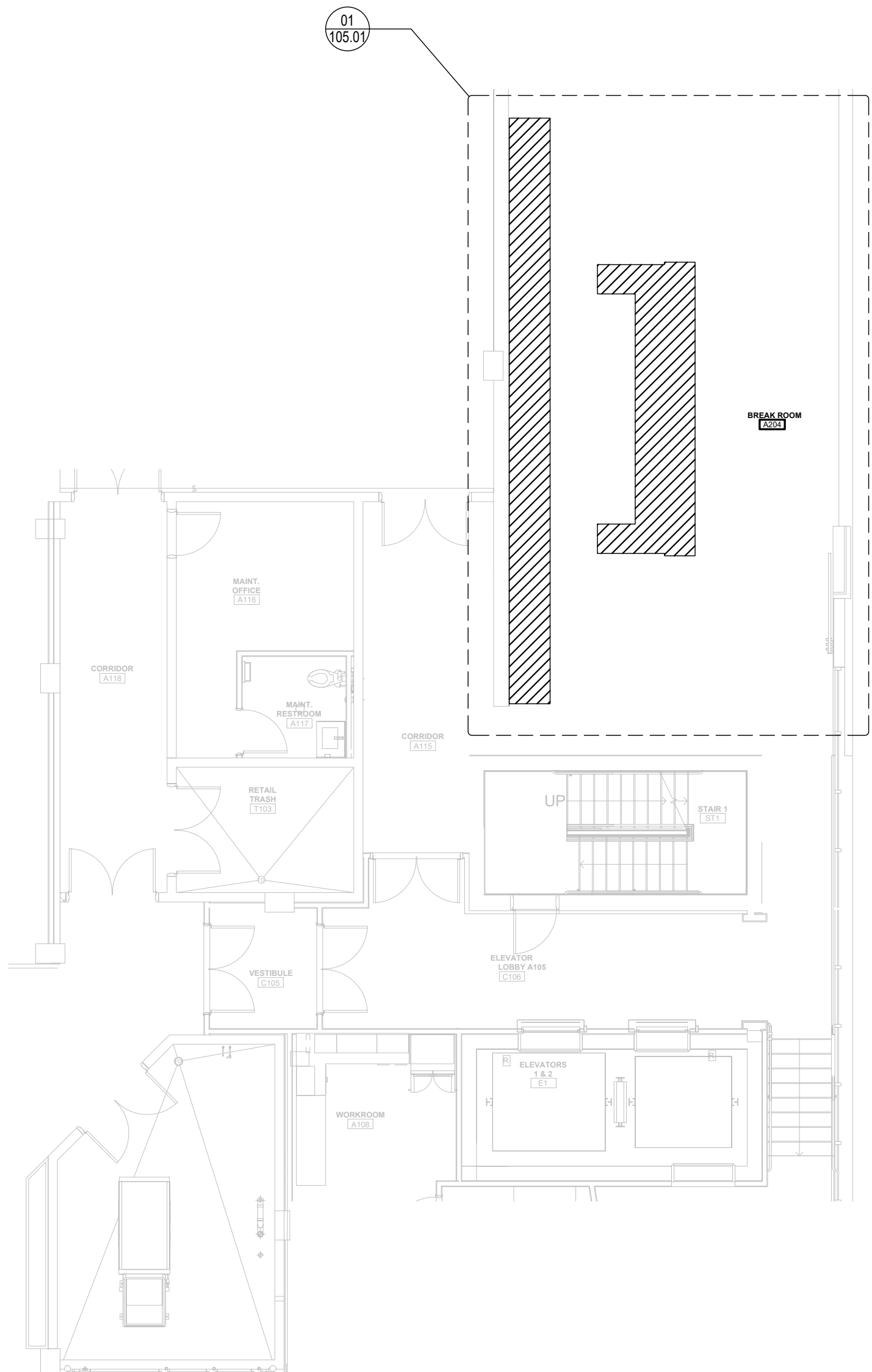
04 LEVEL 1 ENLARGED PLAN - MAIL ROOM REFERENCE PLAN SCALE: 1/8"=1'-0" ARCH REF.: A1/A602A
