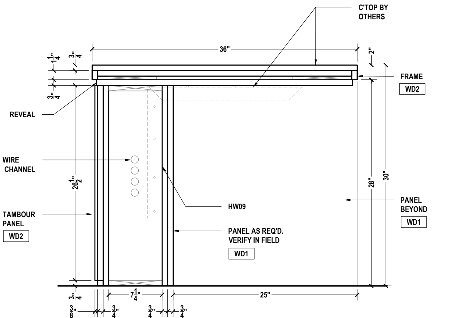
B LOBBY A105 SECTION SCALE: 1-1/2"=1'-0" ARCH REF.: 16/A604B
