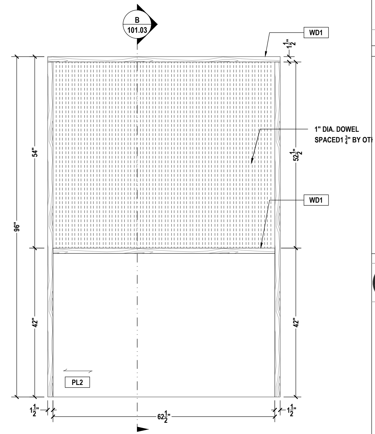
04 LOUNGE A103 - BANQUETTE ELEVATION SCALE: 3/4"=1'-0" ARCH REF.: A4/A603
