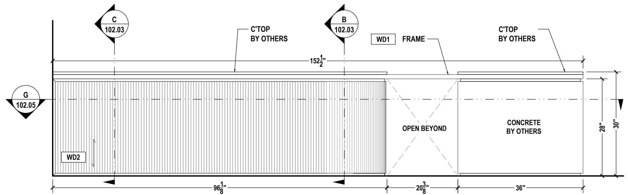
03 LOBBY A105 PLAN VIEW SCALE: 3/4"=1'-0" ARCH REF.: A11/A605
