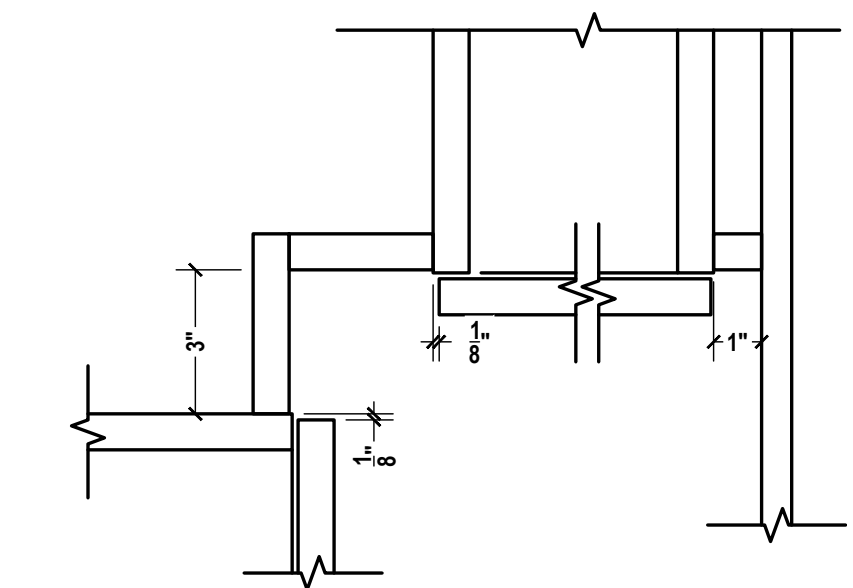
H BASE FILLER / REVEAL DETAIL SCALE: 3"=1'-0" ARCH REF.:
