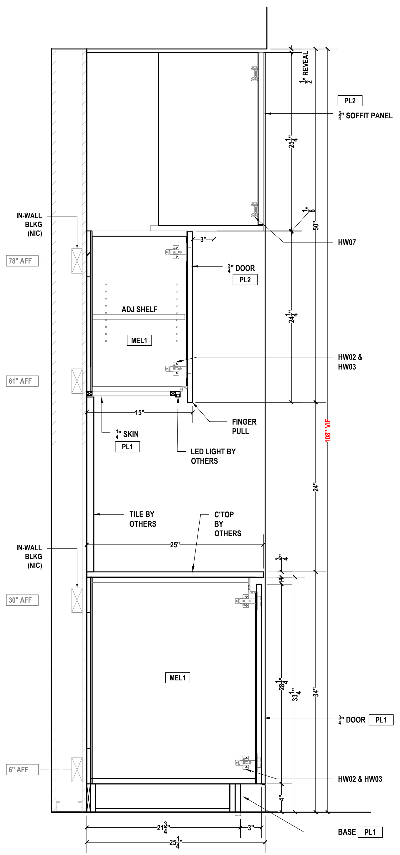
D BREAK ROOM SECTION SCALE: 1-1/2"=1'-0" ARCH REF.: 13/A605B
