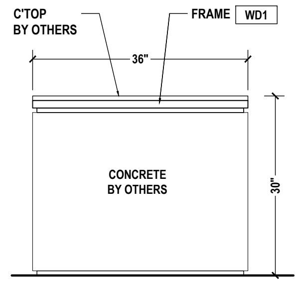
05 LOBBY A105 PLAN VIEW SCALE: 3/4"=1'-0" ARCH REF.: A12/A605
