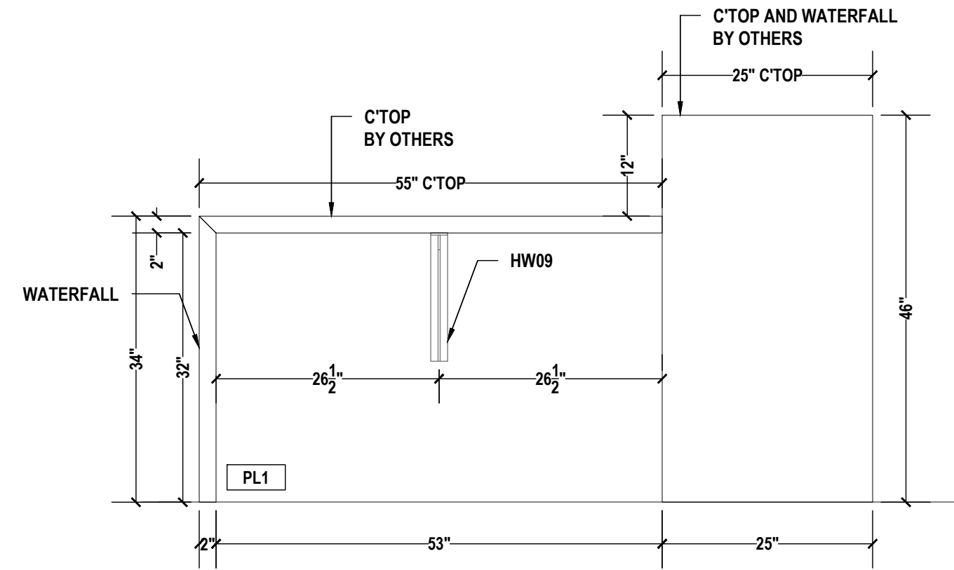
04 BREAK ROOM A204 ELEVATION SCALE: 3/4"=1'-0" ARCH REF.: A3/A608
