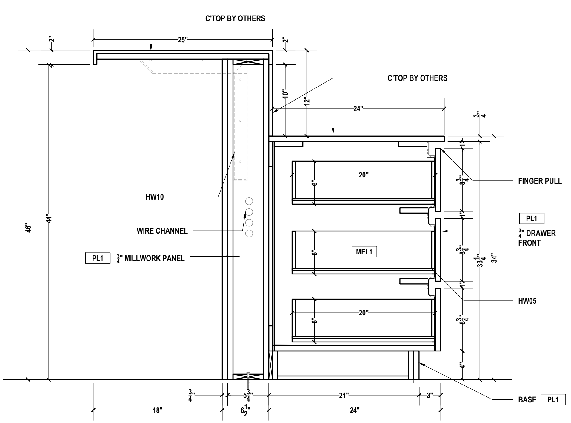
K BREAK ROOM SECTION SCALE: 1-1/2"=1'-0" ARCH REF.: 20/A605B
