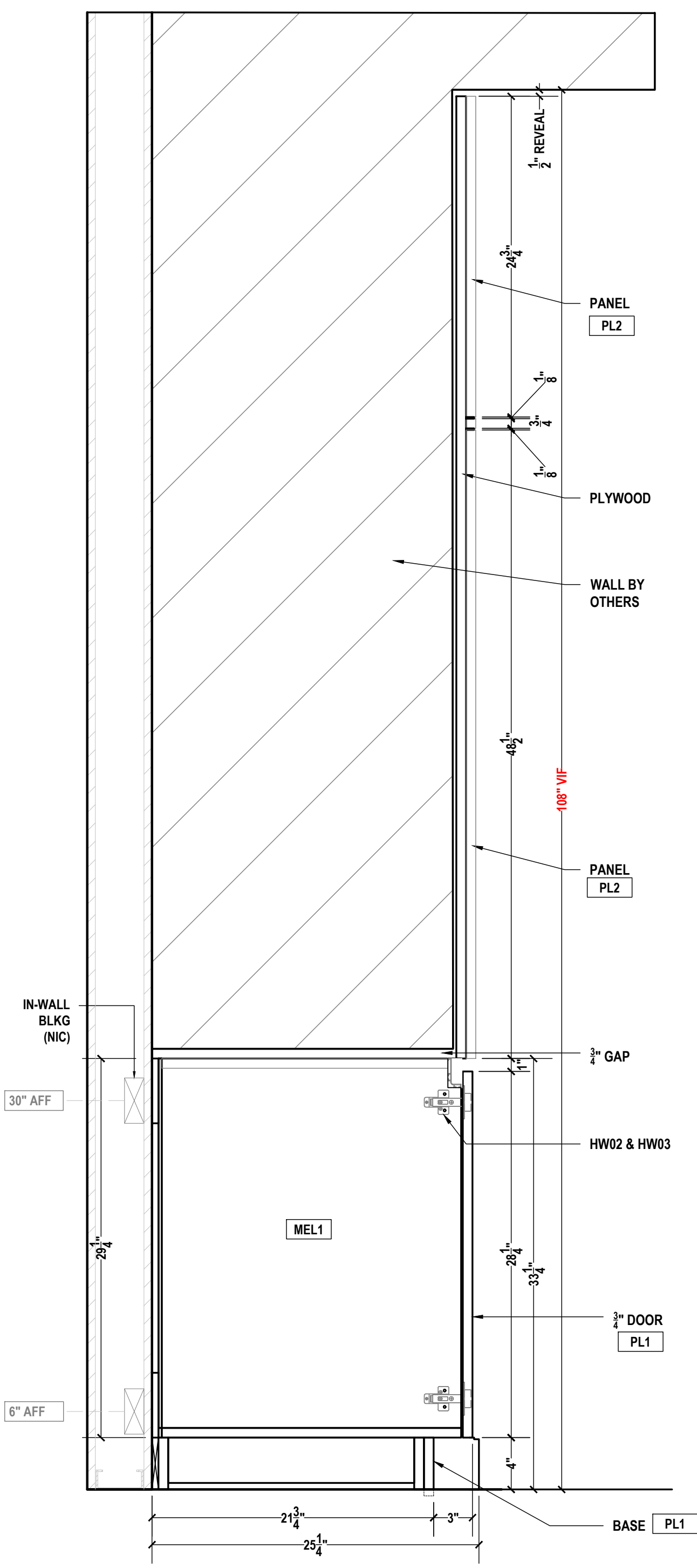
C BREAK ROOM SECTION SCALE: 1-1/2"=1'-0" ARCH REF.: 12/A605B
