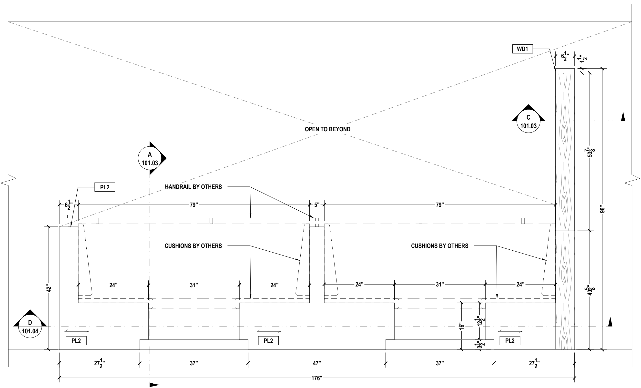
02 LOUNGE A103 - BANQUETTE ELEVATION SCALE: 3/4"=1'-0" ARCH REF.: A2/A603
