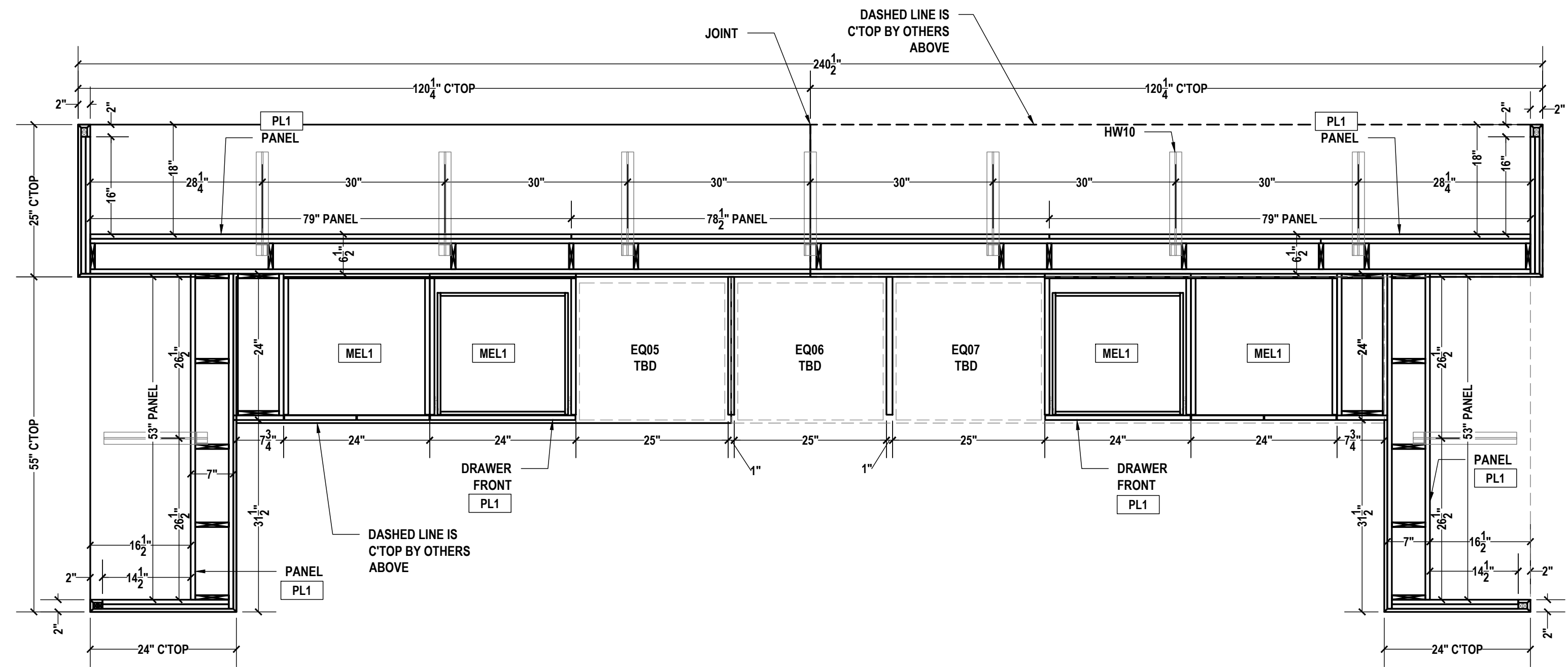
R BREAK ROOM A204 HORIZONTAL SECTION SCALE: 3/4"=1'-0" ARCH REF.: N/A
