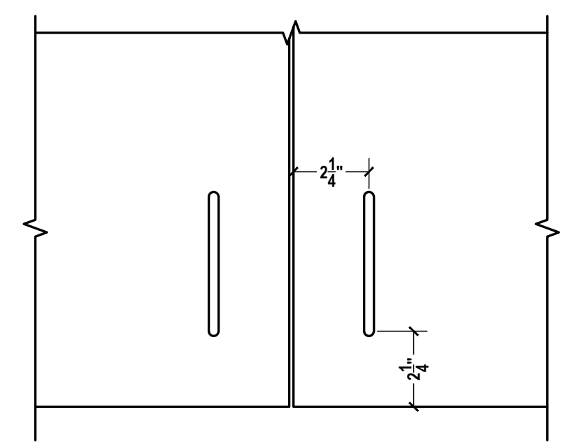
J UPPER DOOR PULL LOCATION DETAIL SCALE: 3"=1'-0" ARCH REF.:
