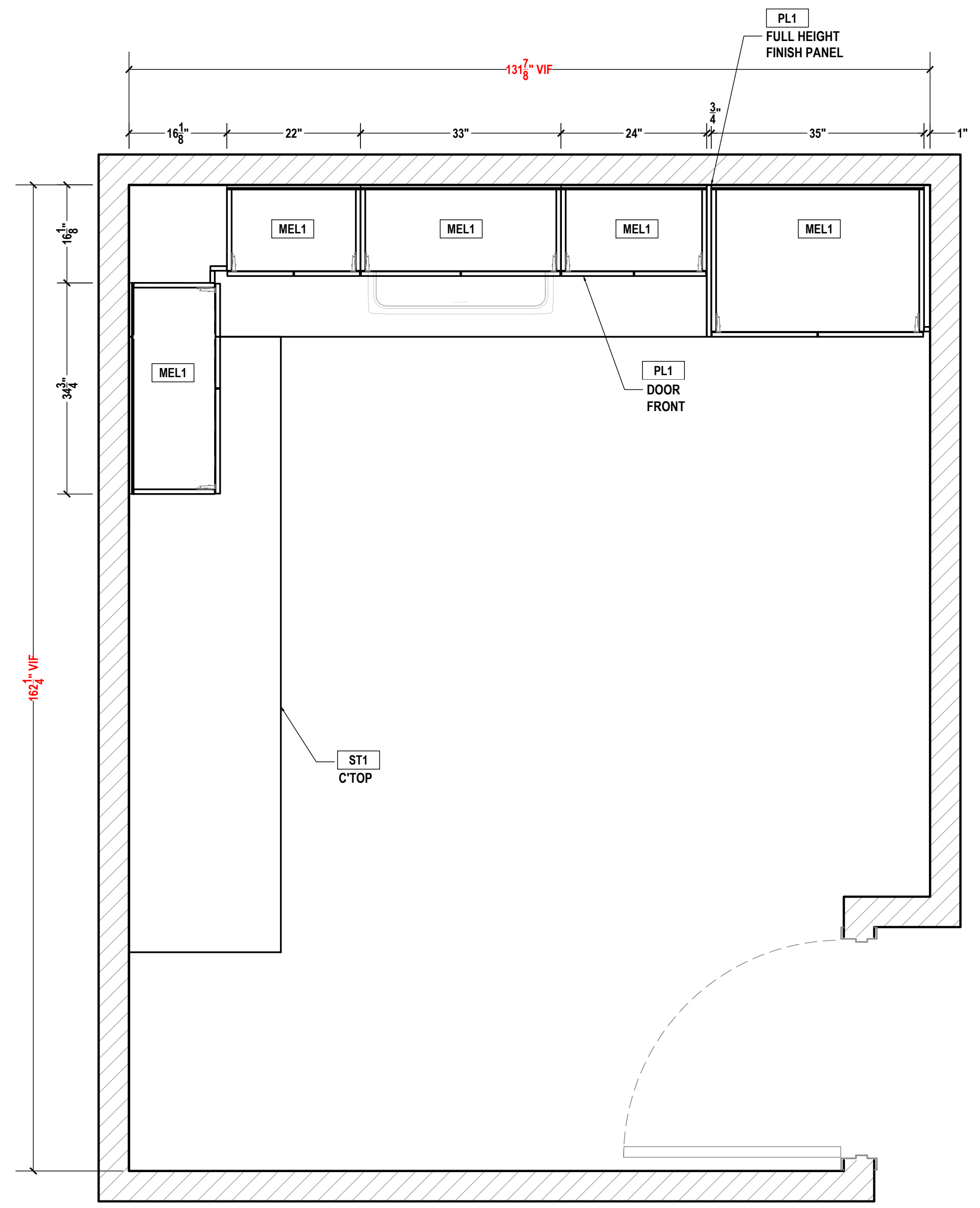
H WORKING ROOM A108 HORIZONTAL SECTION SCALE: 3/4"=1'-0" ARCH REF.: N/A
