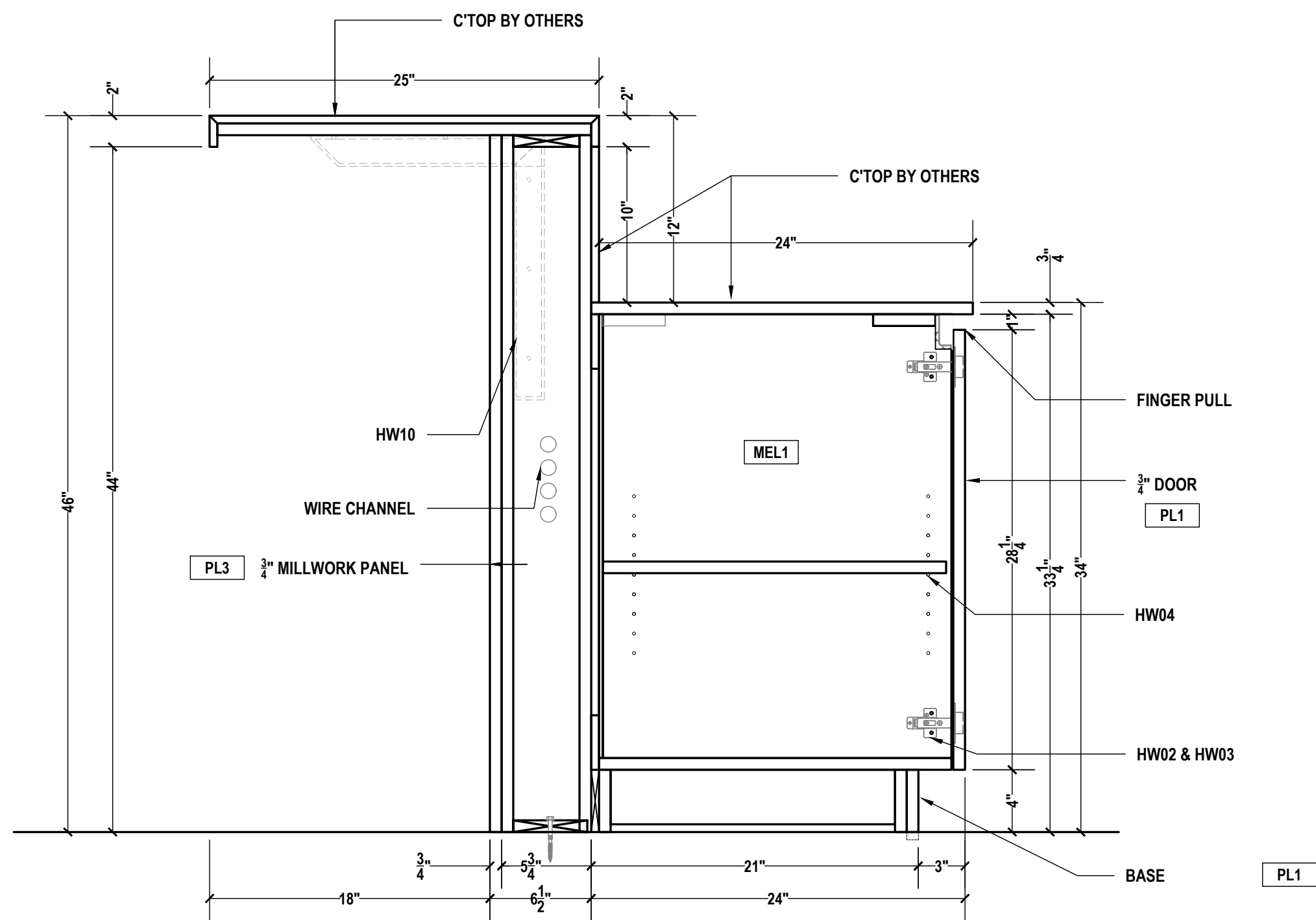
M BREAK ROOM SECTION SCALE: 1-1/2"=1'-0" ARCH REF.: 22/A605B
