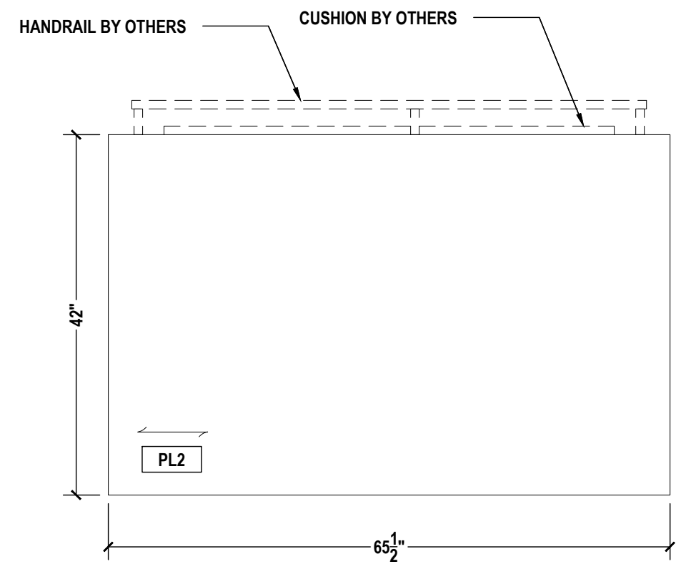
05 LOUNGE A103 - BANQUETTE ELEVATION SCALE: 3/4"=1'-0" ARCH REF.: A5/A603
