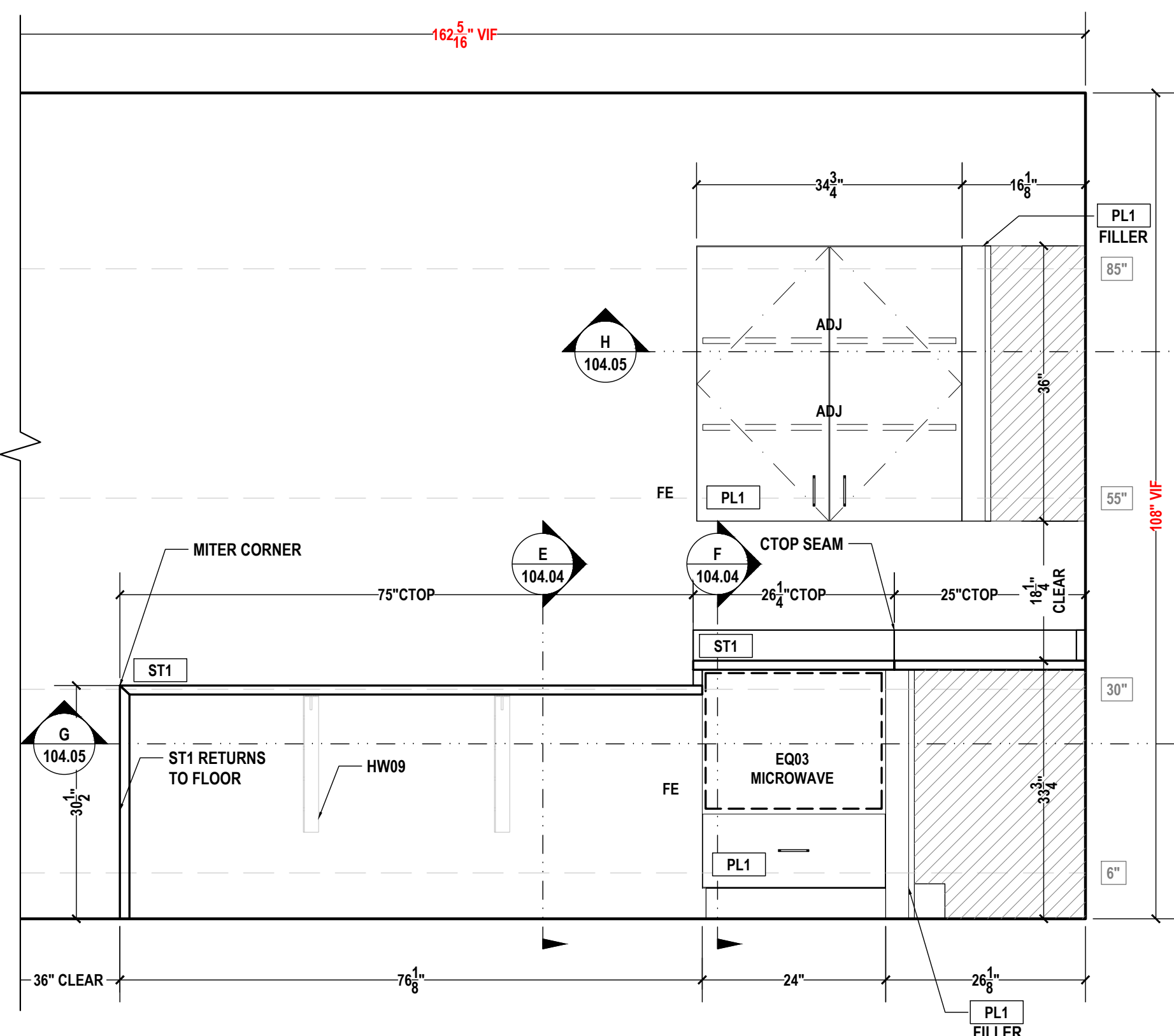
01 WORKING ROOM A108 ELEVATION SCALE: 3/4"=1'-0" ARCH REF.: A3/A607
