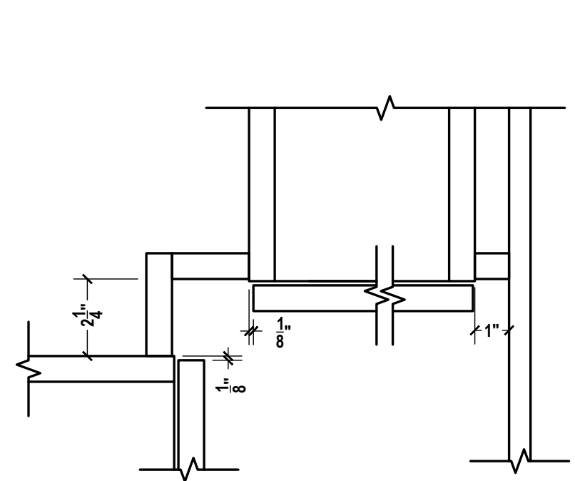
F UPPER FILLER DETAIL SCALE: 3"=1'-0" ARCH REF.:
