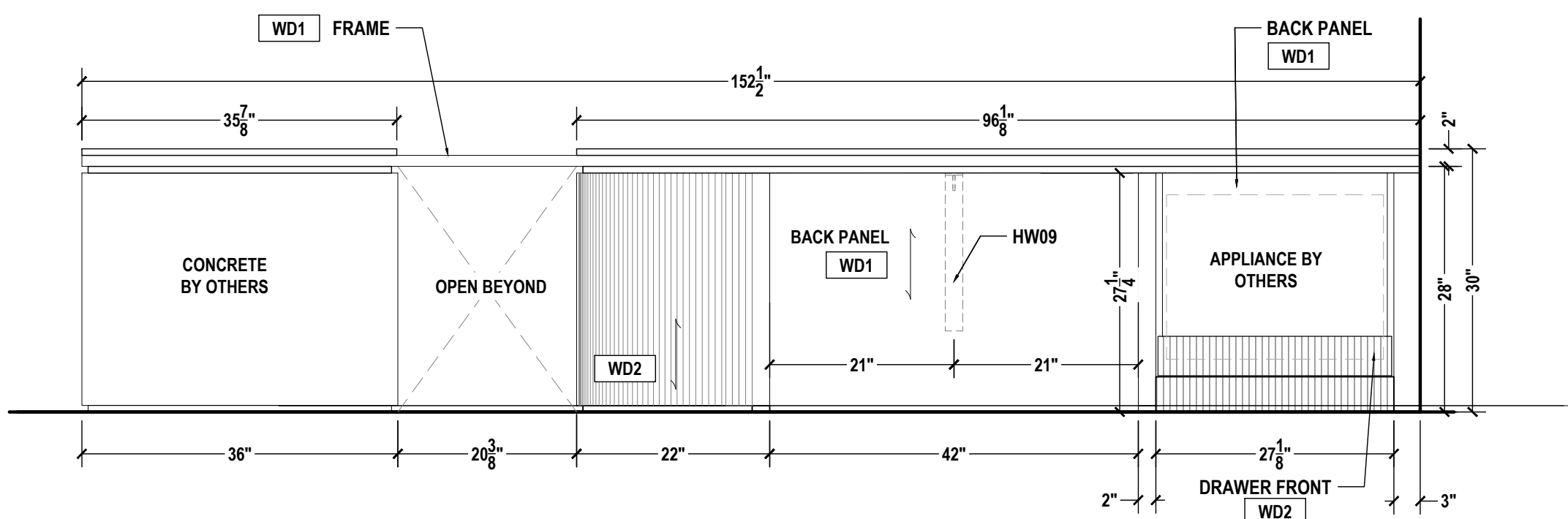
04 LOBBY A105 PLAN VIEW SCALE: 3/4"=1'-0" ARCH REF.: A13/A605
