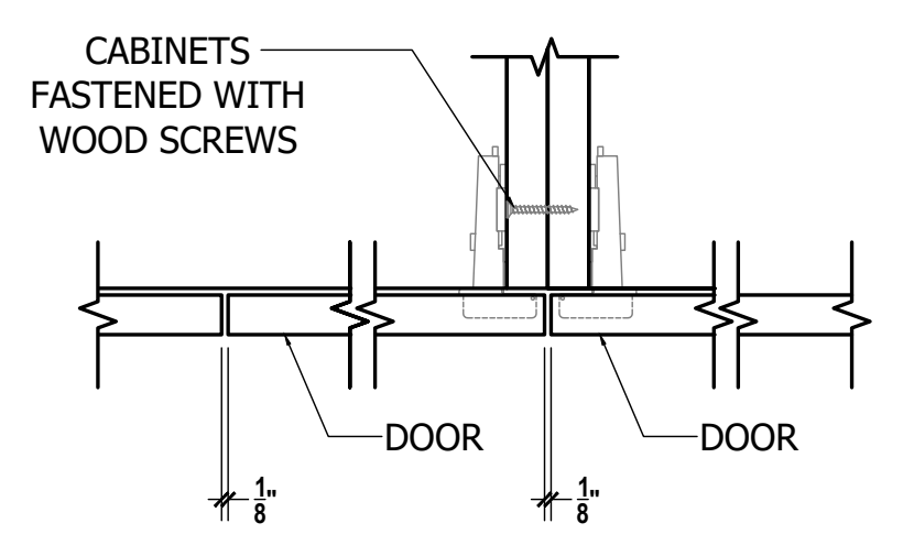
P DOOR GAP DETAIL SCALE: 3"=1'-0" ARCH REF.:
