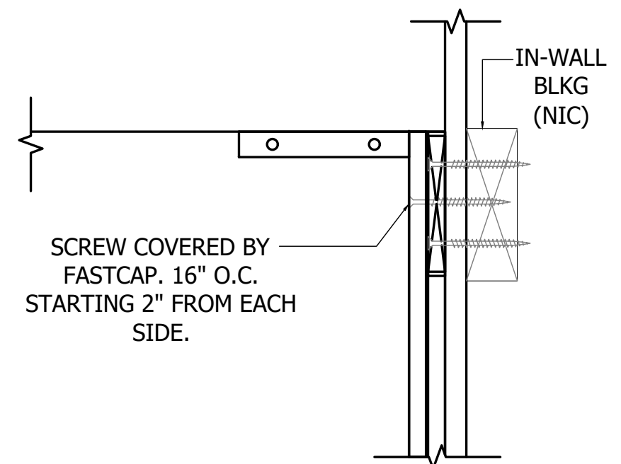
B BASE WALL ANCHORATE DETAIL SCALE: 3"=1'-0" ARCH REF.:
