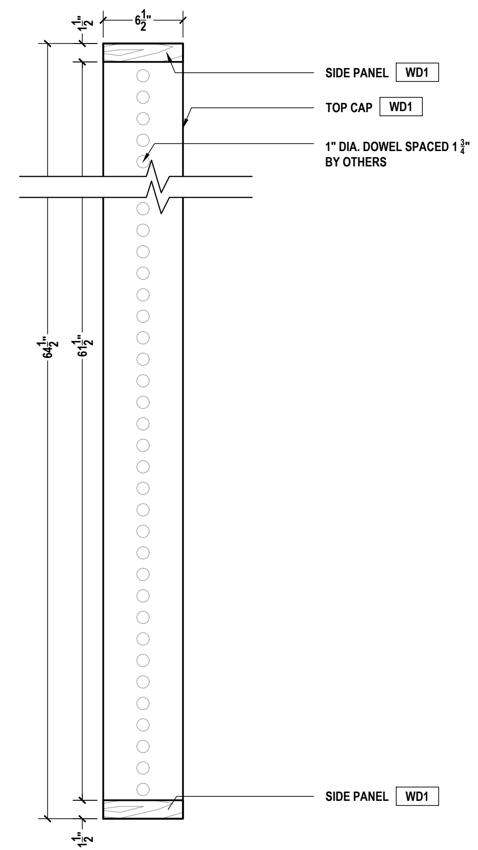
C LOUNGE A103 - BANQUETTE SECTION SCALE: 1-1/2"=1'-0" ARCH REF.: 14/A604B
