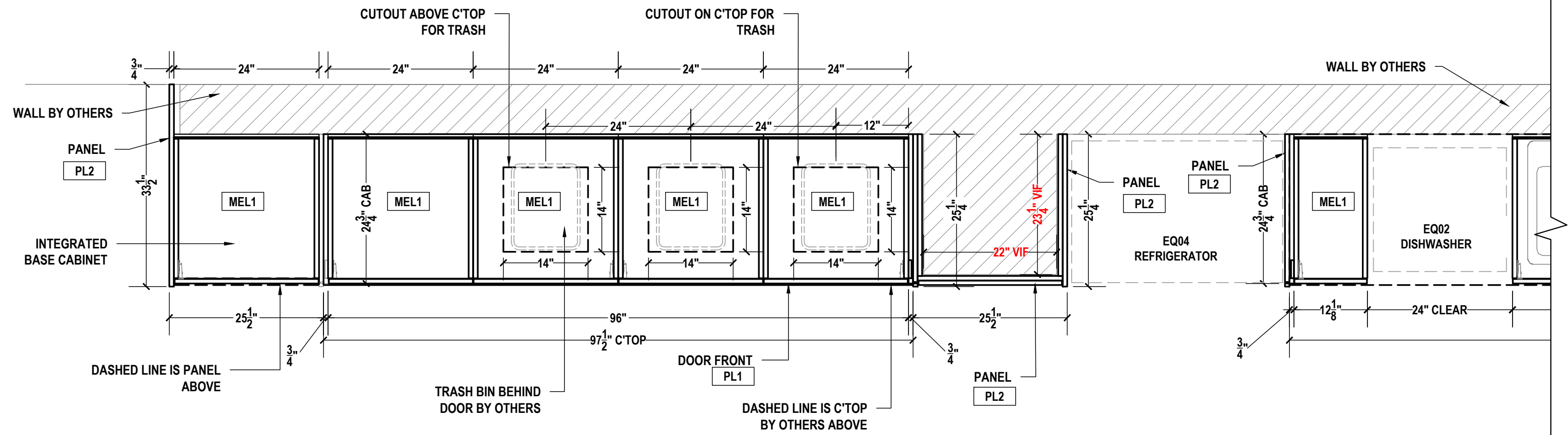
N BREAK ROOM A204 HORIZONTAL SECTION SCALE: 3/4"=1'-0" ARCH REF.: N/A
