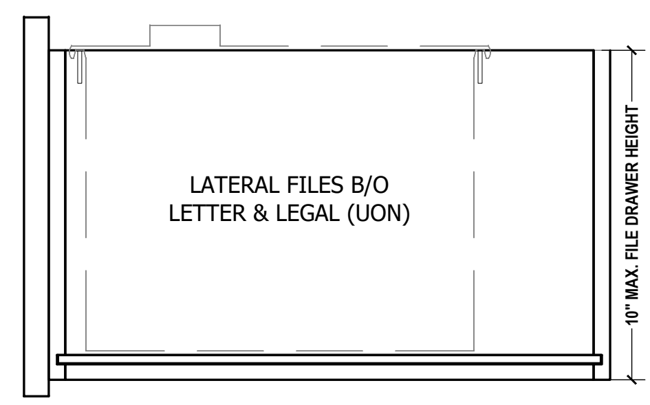
G FILE DRAWER DIMENSIONS DETAIL SCALE: 3"=1'-0" ARCH REF.:
