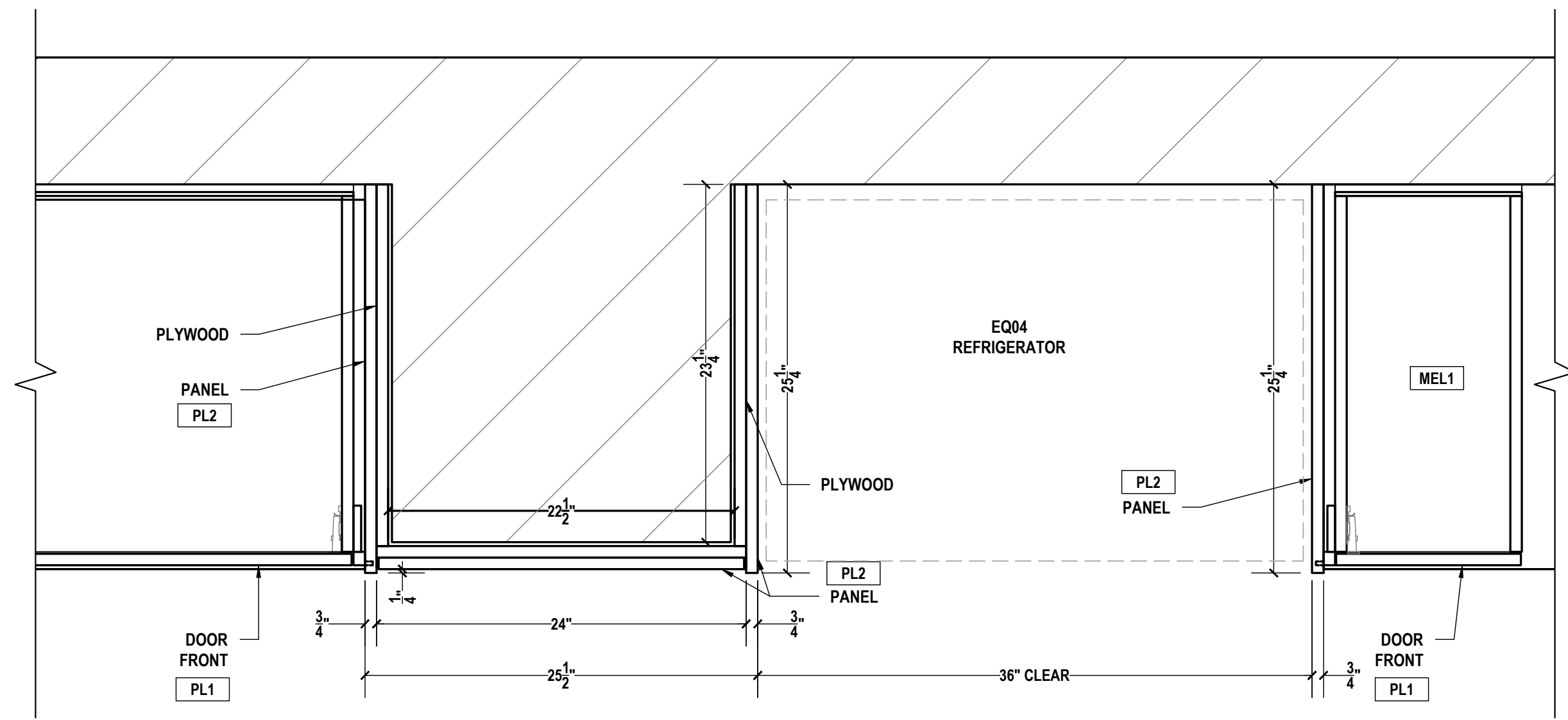
U BREAK ROOM HORIZONTAL SECTION SCALE: 1-1/2"=1'-0" ARCH REF.: 25/A605B
