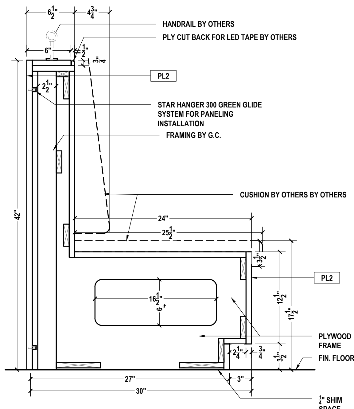
A LOUNGE A103 - BANQUETTE SECTION SCALE: 1-1/2"=1'-0" ARCH REF.: 12/A604B
