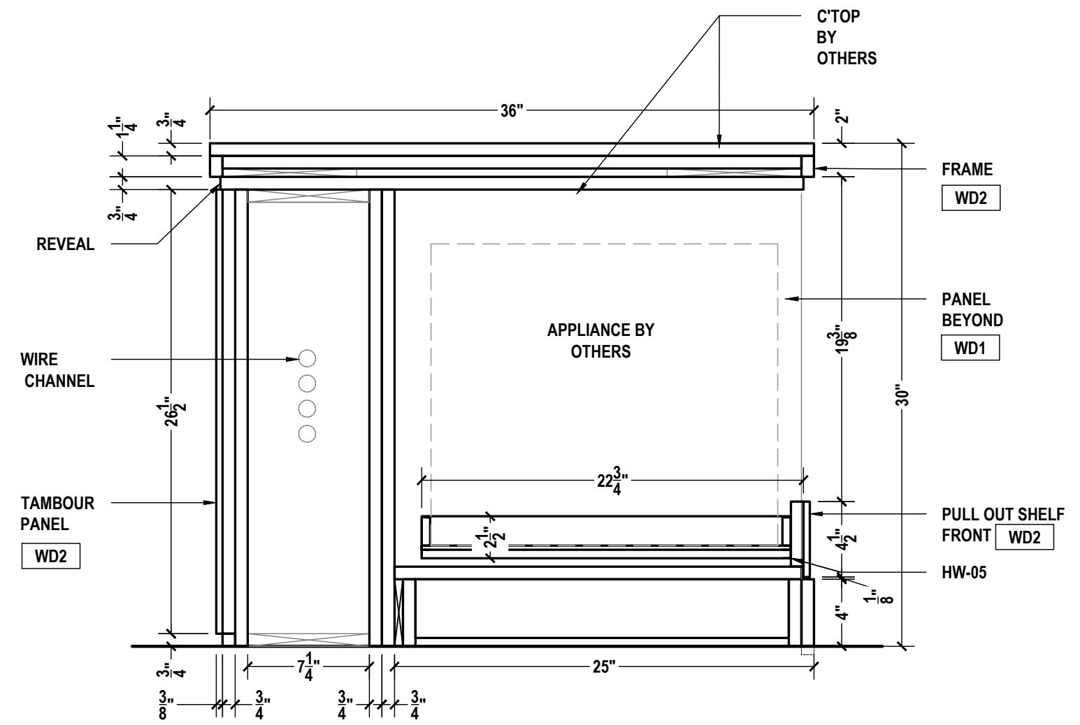
C LOBBY A105 SECTION SCALE: 1-1/2"=1'-0" ARCH REF.: 17/A604B
