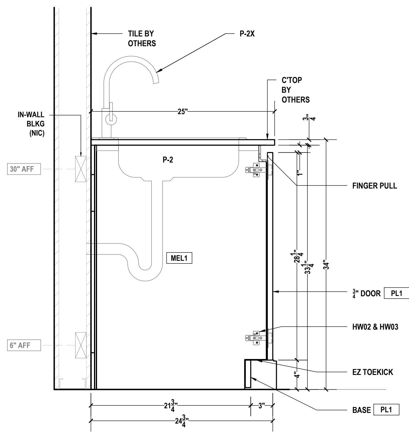
F BREAK ROOM SECTION SCALE: 1-1/2"=1'-0" ARCH REF.: 15/A605B
