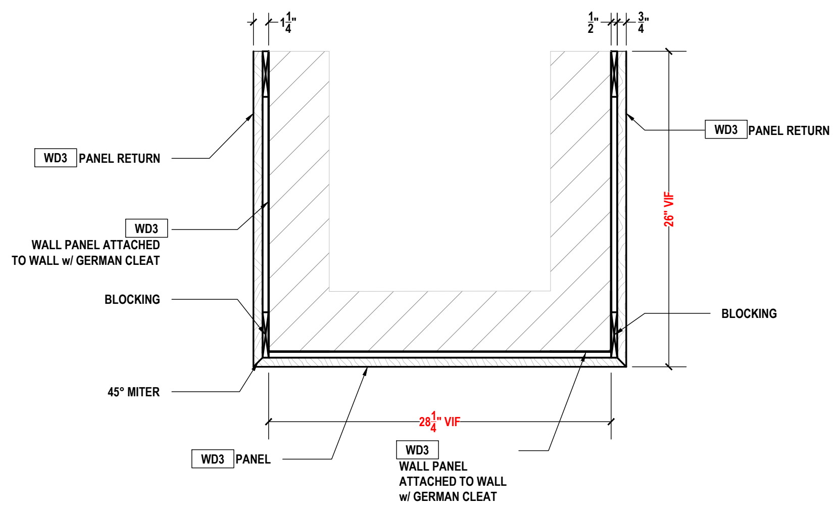
C RESTROOMS A402 HORIZONTAL SECTION SCALE: 1-1/2"=1'-0" ARCH REF.: 20/A604B
