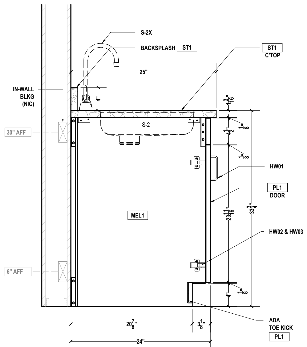
B WORKING ROOM A108 SECTION SCALE: 1-1/2"=1'-0" ARCH REF.: 22/A604B
