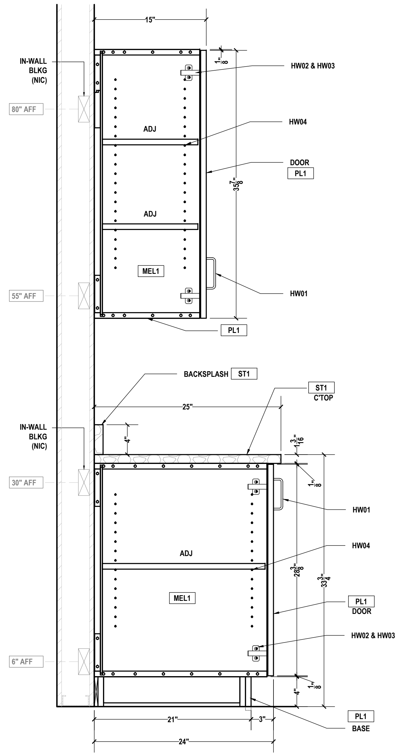
A WORKING ROOM A108 SECTION SCALE: 1-1/2"=1'-0" ARCH REF.: 21/A604B
