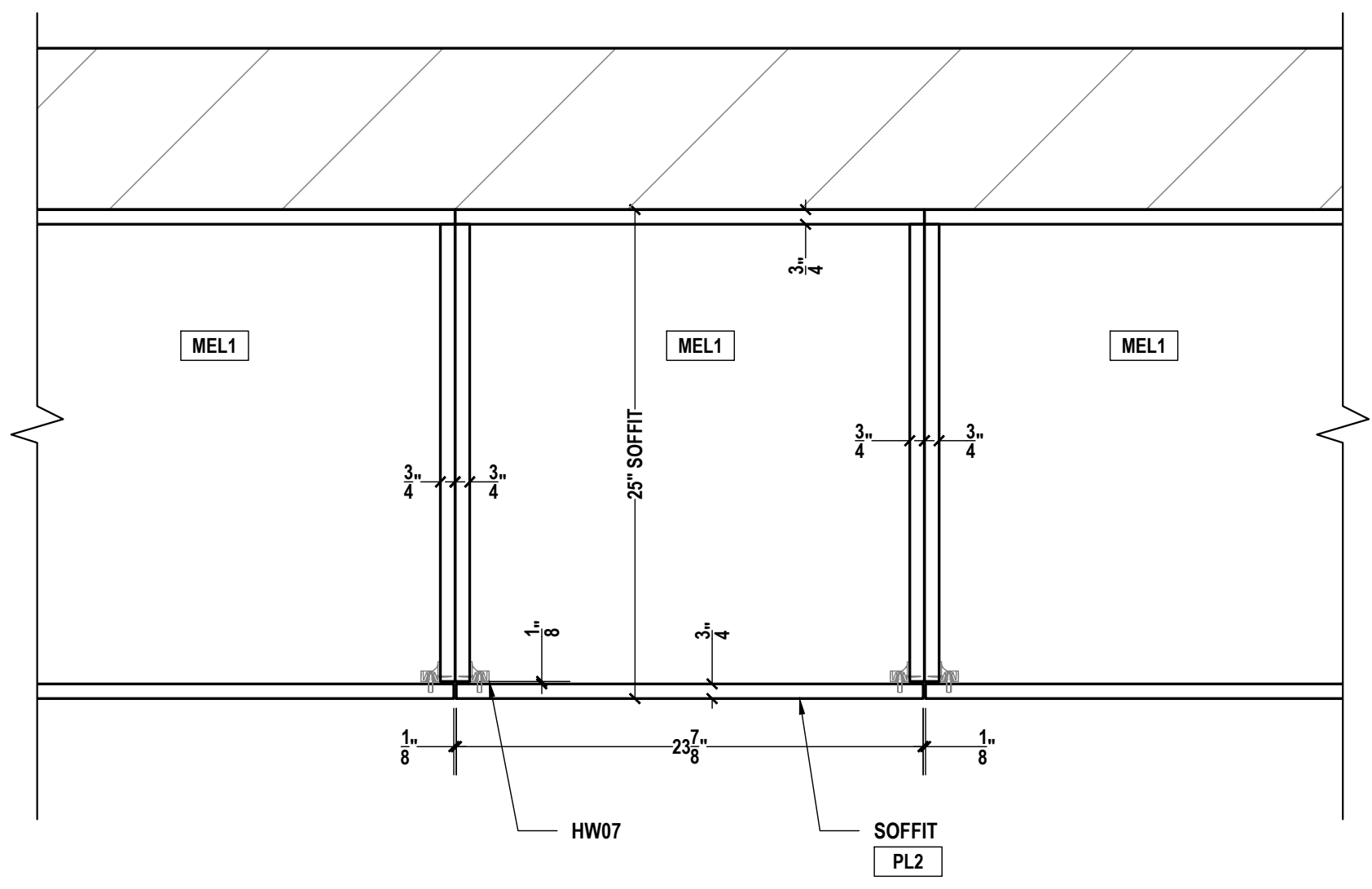
T BREAK ROOM HORIZONTAL SECTION SCALE: 1-1/2"=1'-0" ARCH REF.: 24/A605B
