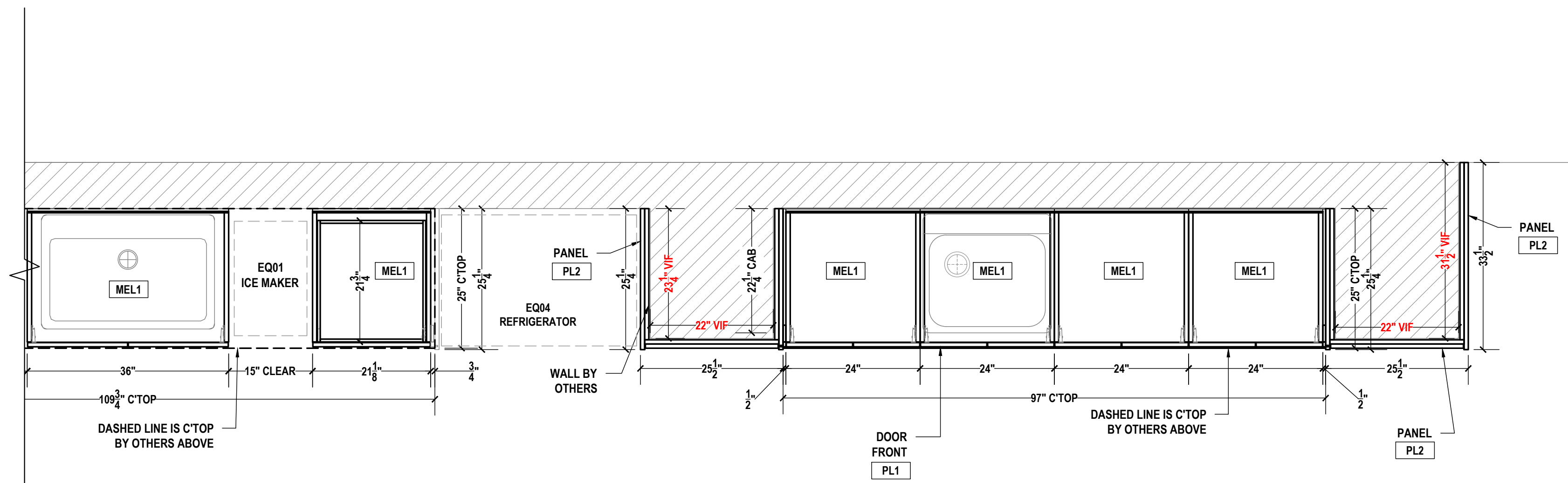
O BREAK ROOM A204 HORIZONTAL SECTION SCALE: 3/4"=1'-0" ARCH REF.: N/A
