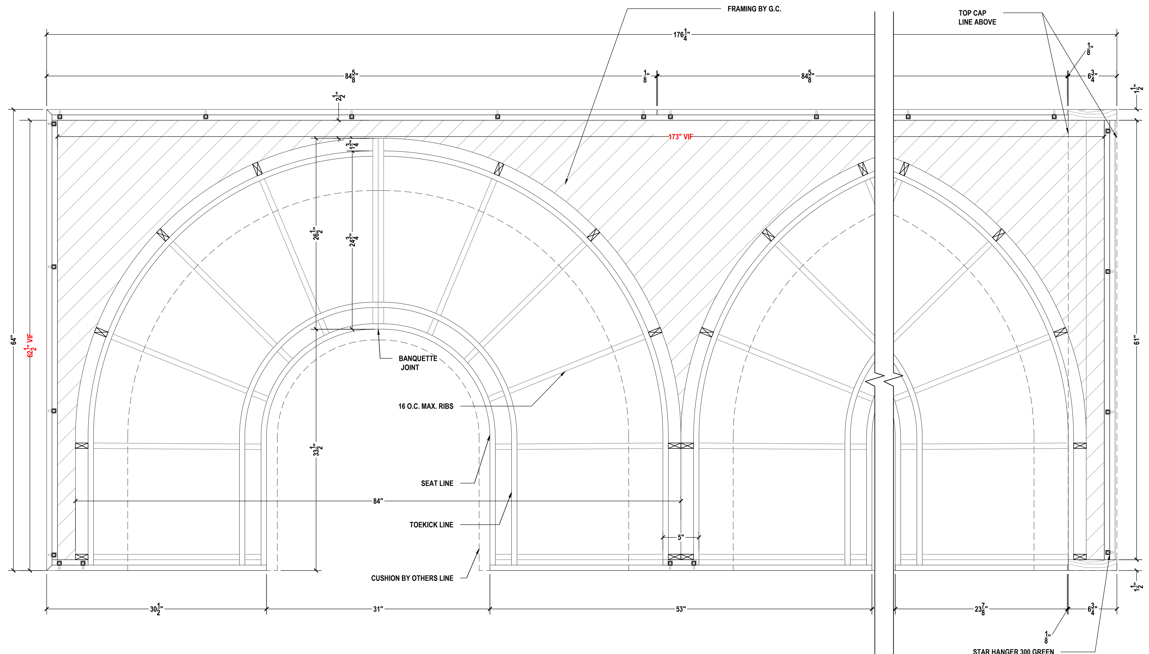
D LOUNGE A103 - BANQUETTE PLAN SECTION SCALE: 1-1/2"=1'-0" ARCH REF.: N/A
