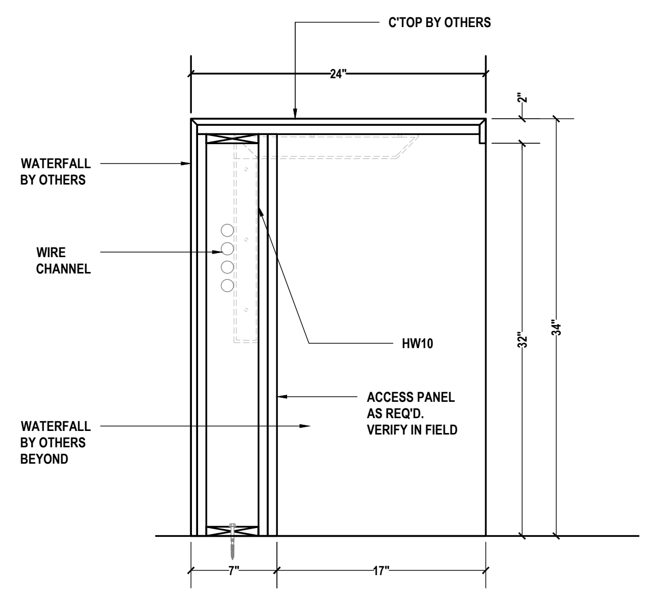
L BREAK ROOM SECTION SCALE: 1-1/2"=1'-0" ARCH REF.: 21/A605B
