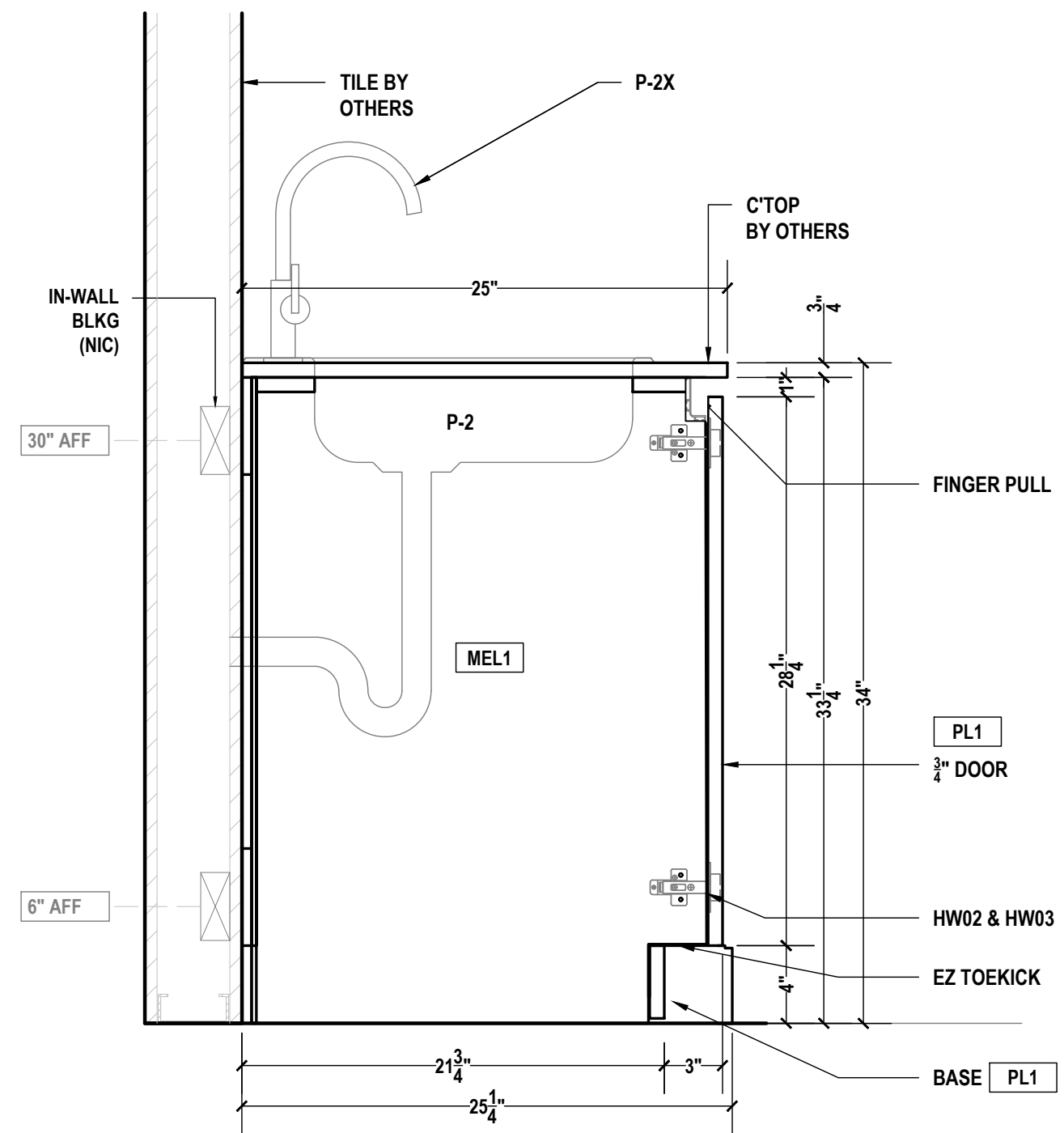
H BREAK ROOM SECTION SCALE: 1-1/2"=1'-0" ARCH REF.: 17/A605B
