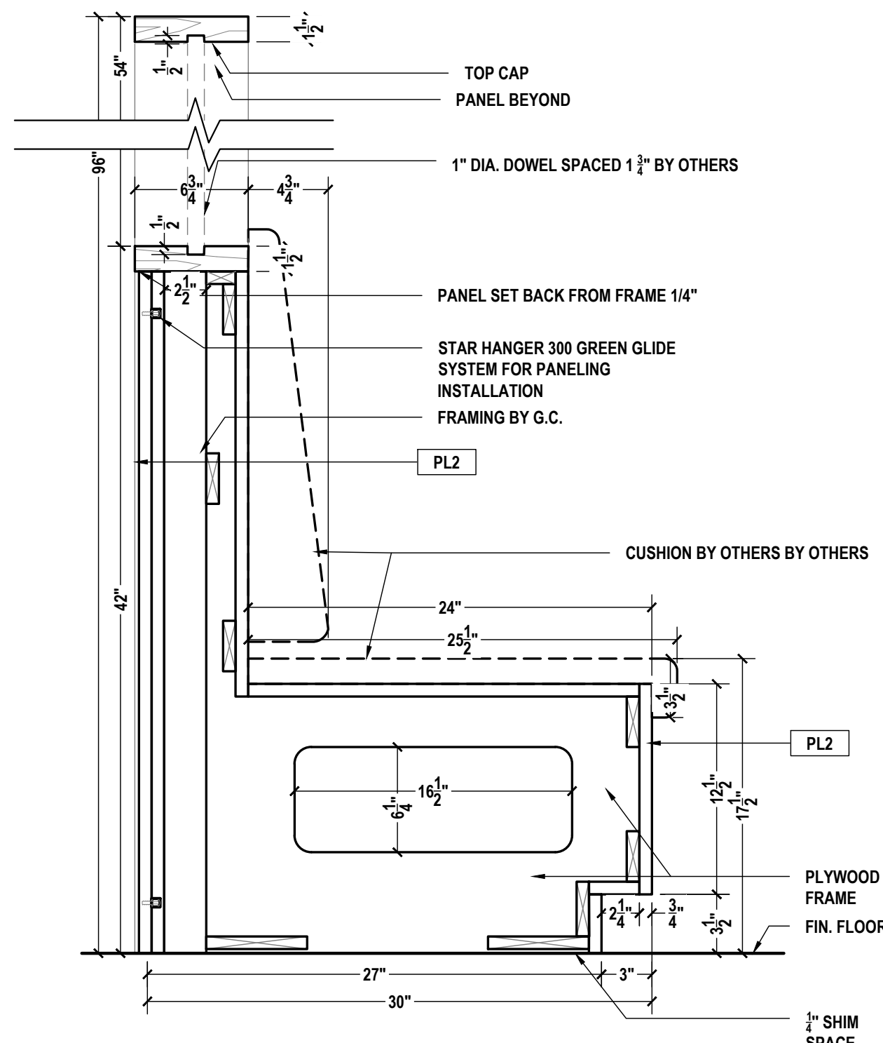
B LOUNGE A103 - BANQUETTE SECTION SCALE: 1-1/2"=1'-0" ARCH REF.: 13/A604B
