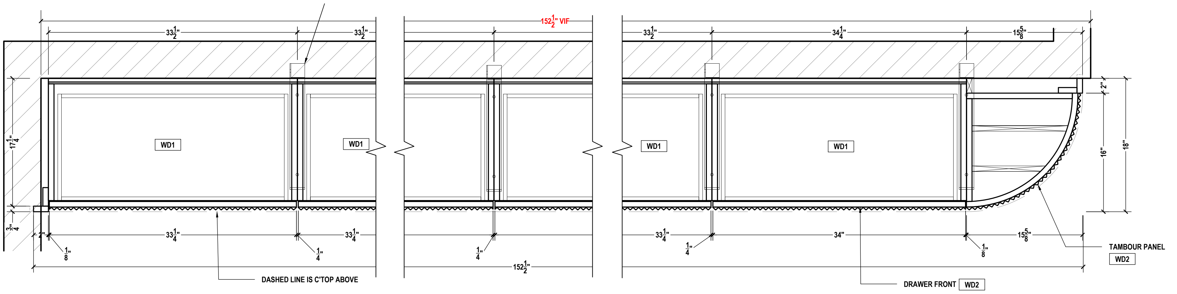
F LOBBY A105 HORIZONTAL SECTION SCALE: 1-1/2"=1'-0" ARCH REF.: N/A
