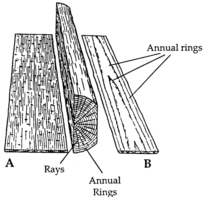
Figure 4. (A) Edgegrained or quartersawn (B) Flatsawn the same kinds of wood. Figure 4 illustrates how wood grain in boards can be altered by the way the board is cut from a log.
